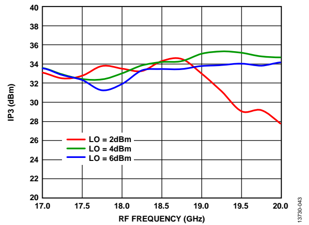
Figure 43. Output IP3 vs. RF Frequency at Various LO Powers
