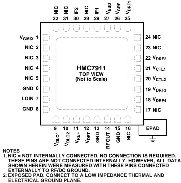
Figure 2. Pin Configuration
