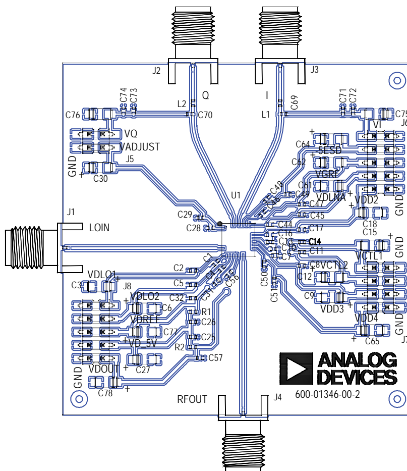
Figure 84. Evaluation Board Top Layer
