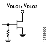
Figure 6. V_{DLO1} , V_{DLO2} Interface
