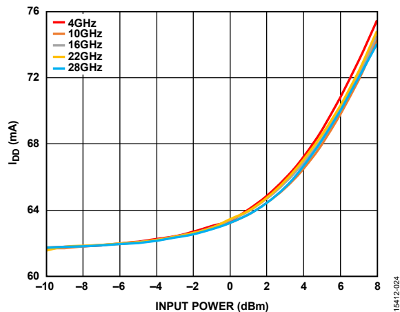
Figure 24. I_{DD} vs. Input Power at Various Frequencies
