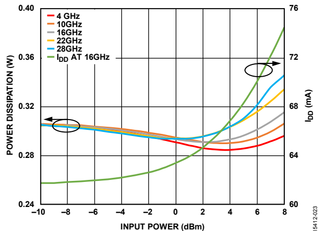
Figure 23. Power Dissipation and I_{DD} vs. Input Power at Various Frequencies, 16 GHz, T_A = 85^\circ C
