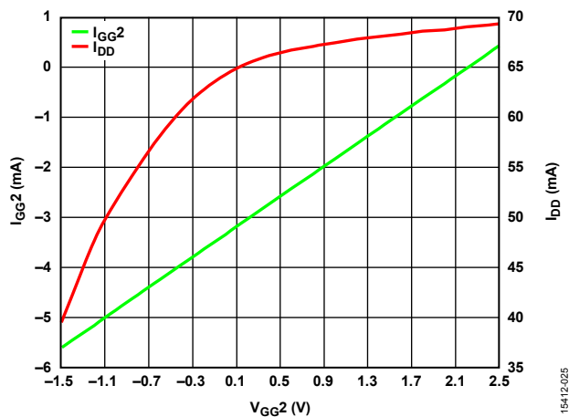
Figure 25. I_{GG2} and I_{DD} vs. V_{GG2} at 14 GHz, Input Power ( P_{IN} ) = 0 dBm
