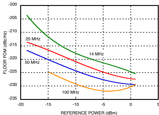
Figure 11. Reference Input Sensitivity Sinusoid Wave, 50 \Omega [3]
