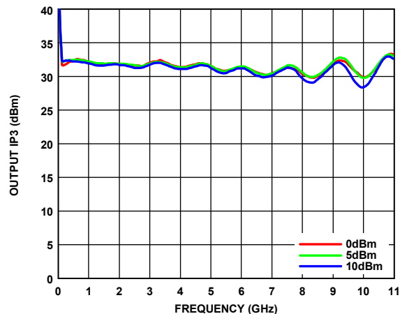
Figure 17. Output IP3 vs. Frequency for Various P_{OUT}/Tone
