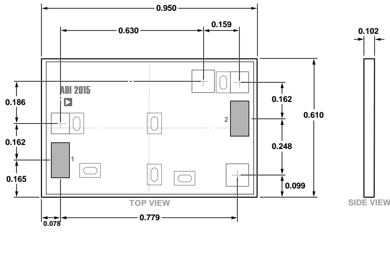
Figure 42. 2-Pad Bare Die [CHIP] (C-2-3) Dimensions shown in millimeters
