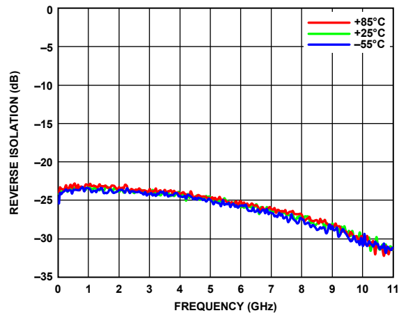
Figure 16. Reverse Isolation vs. Frequency for Various Temperatures
