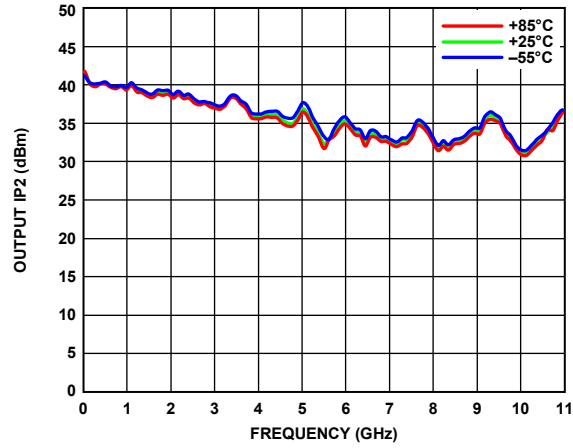
Figure 15. Output IP2 vs. Frequency for Various Temperatures at P_{OUT}/Tone = 5 \text{ dBm}
