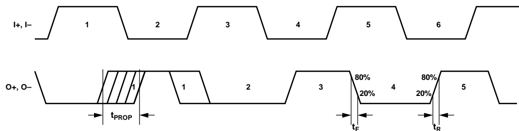
Figure 2. Timing Diagram
