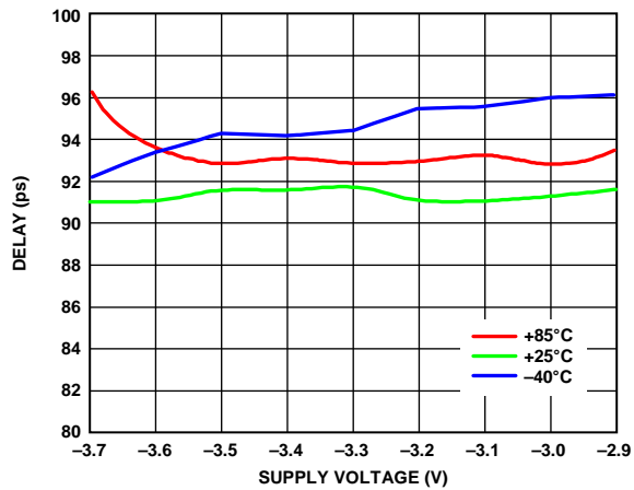
Figure 15. Delay vs. Supply Voltage at Various Temperatures
