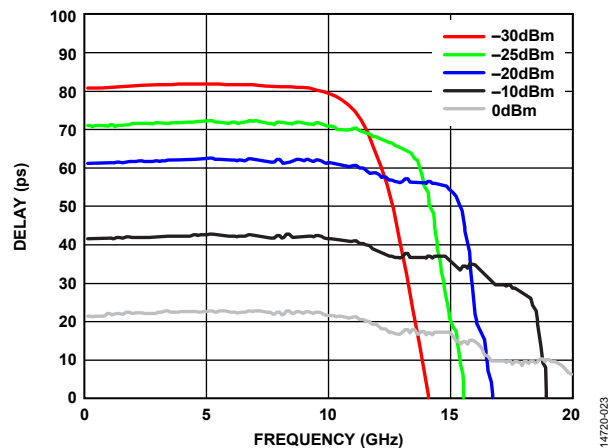
Figure 23. Delay vs. Frequency at Various Input Powers (Device Measured on an Evaluation Board with Port Extensions)
