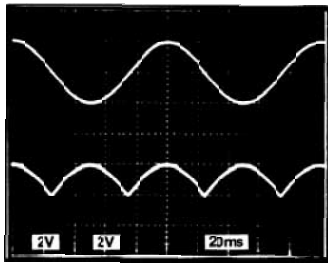
Figure 8. Output of Full-Wave Rectifier with 4 V p-pr 10 Hz Input
