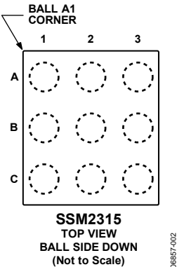
Figure 2. Pin Configuration
