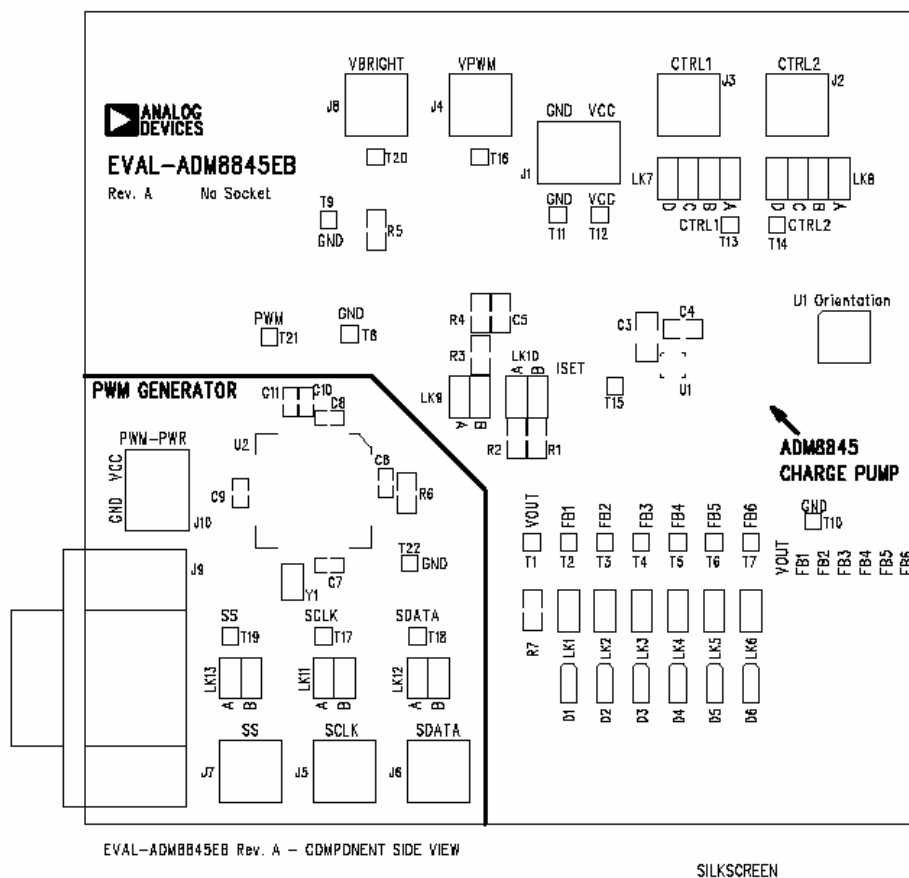
Figure 6. ADM8845 Evaluation Board Silkscreen
