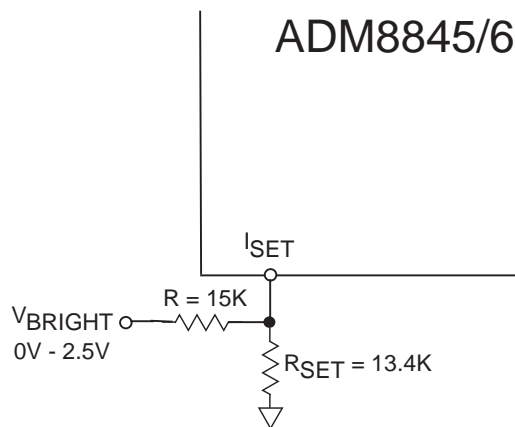
Figure 8. V_{BRIGHT} Node
