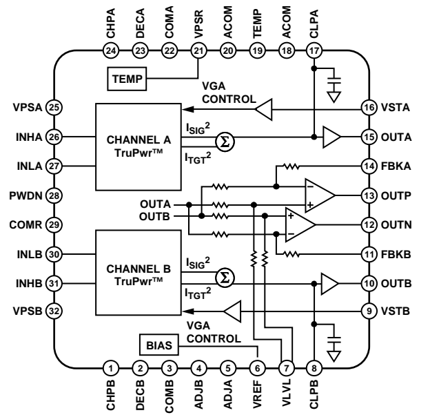
Figure 59. Op Amp Connections (All Resistors are 1 kΩ ± 20%)
