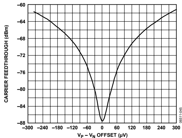
Figure 26. Carrier Feedthrough vs. DC Offset Voltage at 1900 MHz
