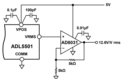
Figure 47. Output Buffering Options, Slope of 12.6 V/V rms at 900 MHz
