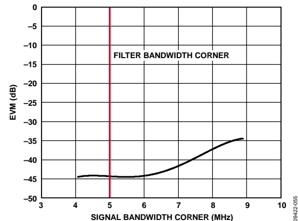
Figure 53. EVM vs. Signal Bandwidth Corner at a Filter Corner of 5 MHz and a 16-QAM Signal with a = 0.35
