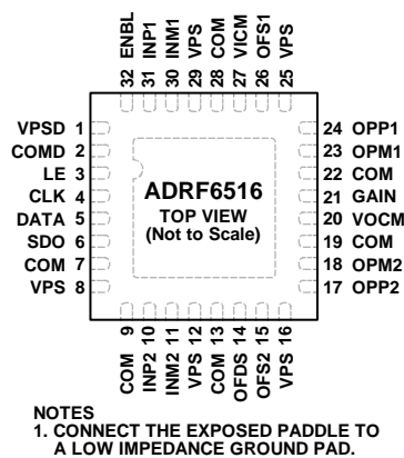
Figure 4. Pin Configuration
