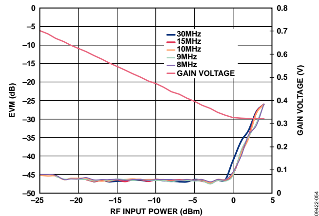
Figure 52. EVM vs. RF Input Power at Several Filter Corner Settings (256-QAM, 14 MSPS Signal with a = 0.35 ; Output Differential Signal Level Held to 700 mV p-p; OFDS Pulled High)
