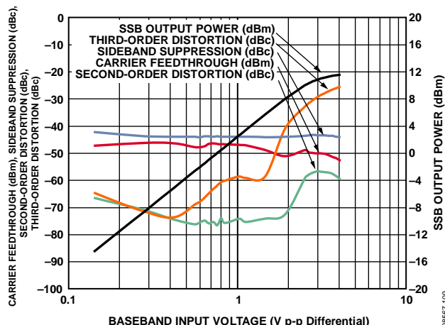
Figure 9. SSB Output Power, Second- and Third-Order Distortion, Carrier Feedthrough and Sideband Suppression vs. Baseband Differential Input Voltage ( f_{\text{OUT}} = 1100\text{ MHz} )
