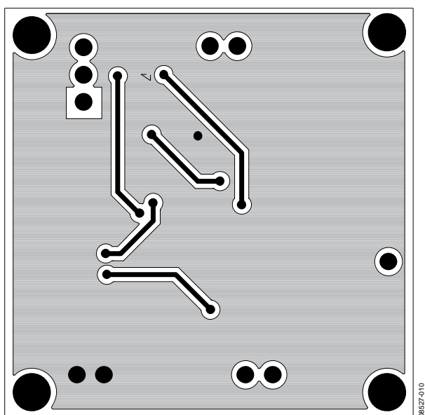
Figure 9. ADP1612/ADP1613 Boost Application PCB Bottom Layer
