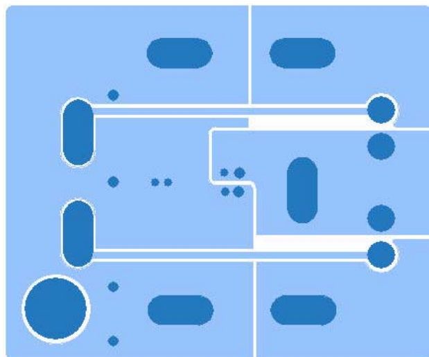
Figure 10. Typical Board Layout, Bottom Side
