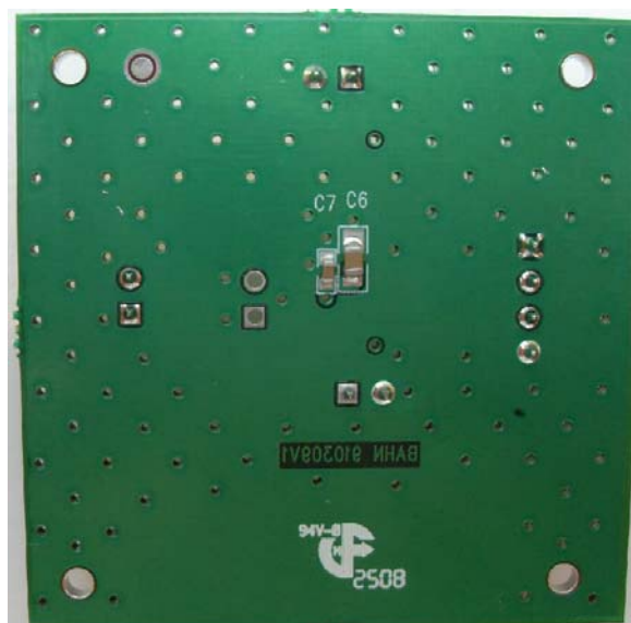
Figure 2. SSM2335 Evaluation Board, Bottom View
