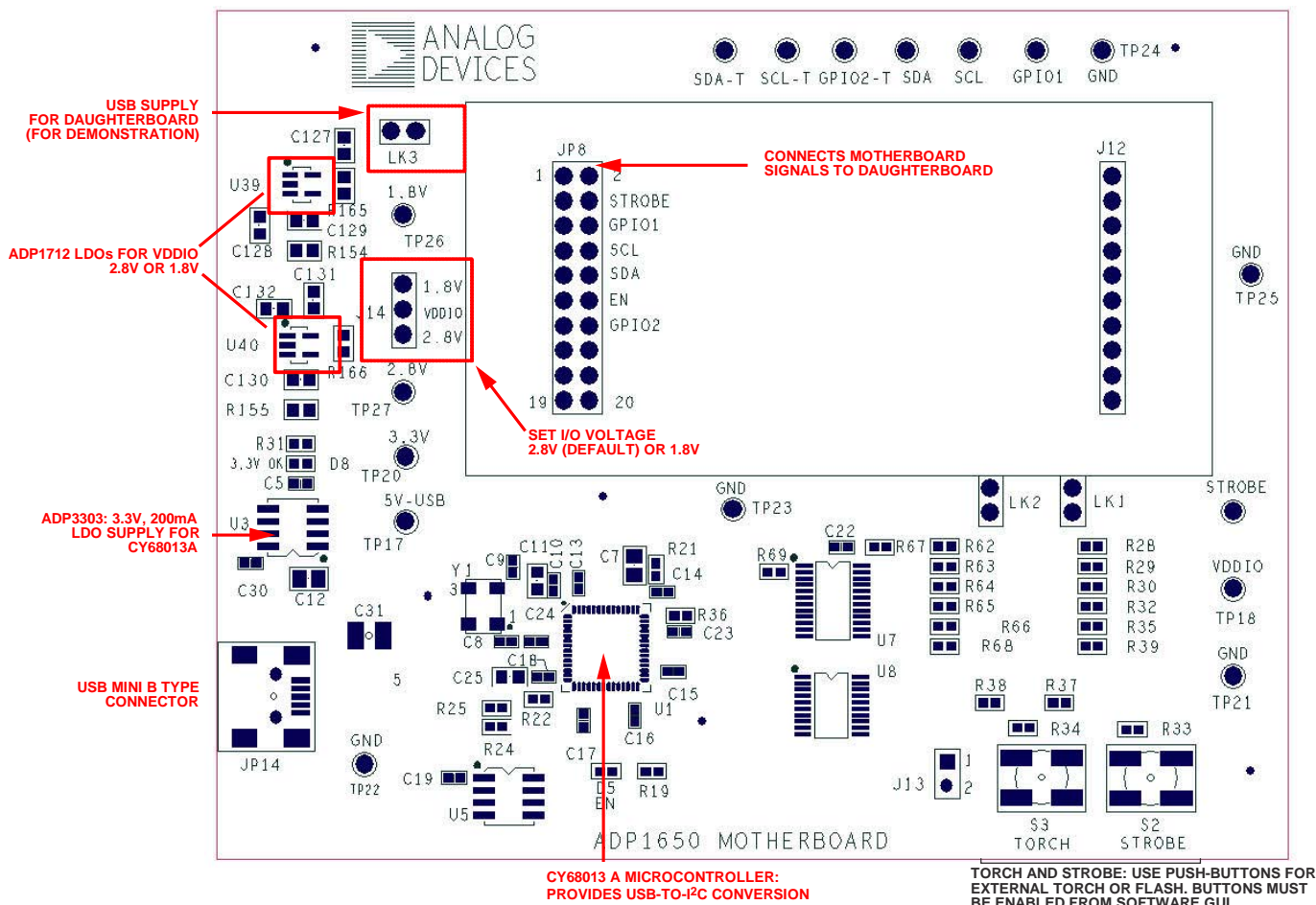
Figure 9. Motherboard
