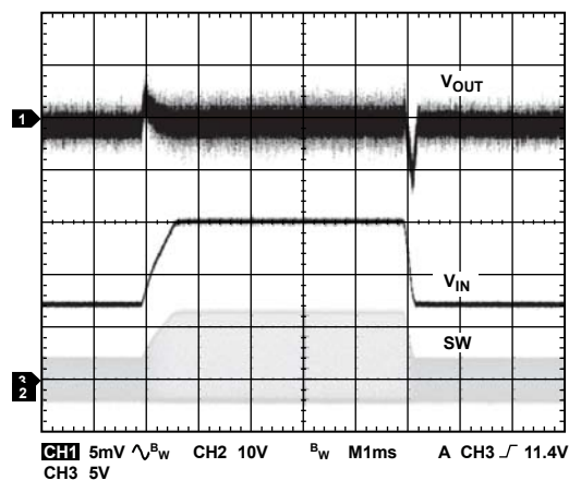
Figure 11. ADP2301 Line Transient, 7 V to 15 V, V_{OUT} = 3.3 V, I_{OUT} = 1.2 A, f_{SW} = 1.4 MHz
