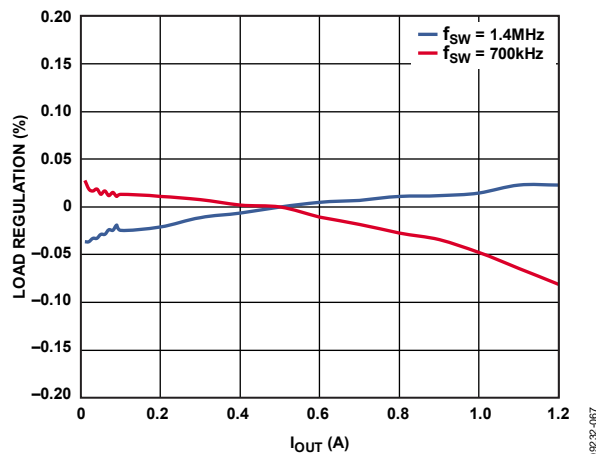
Figure 5. Load Regulation, V_{OUT} = 3.3V , V_{IN} = 12V
