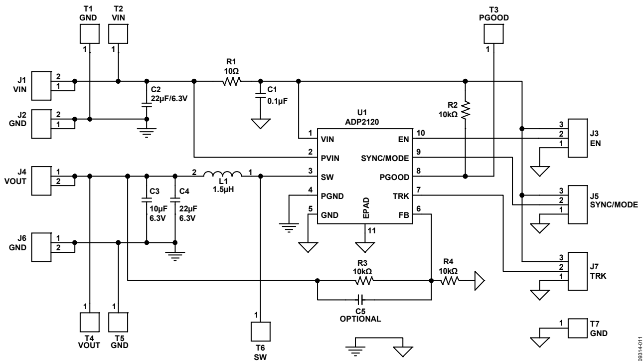
Figure 11. ADP2120 Evaluation Board Schematic
