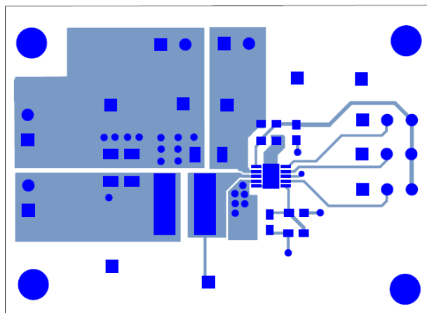
Figure 12. Top Layer
