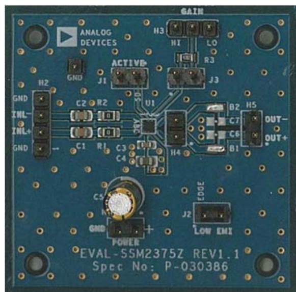
Figure 1. SSM2375 Evaluation Board Top View
