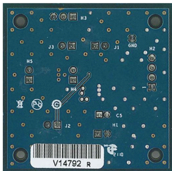
Figure 2. SSM2375 Evaluation Board Bottom View
