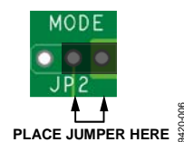
Figure 6. PWM Mode Jumper Position
