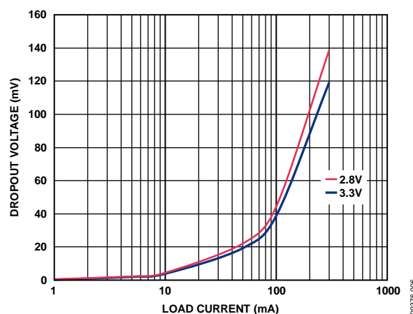
Figure 6. Dropout Voltage vs. Load Current, V_{OUT} = 2.8\text{ V} and V_{OUT} = 3.3\text{ V}
