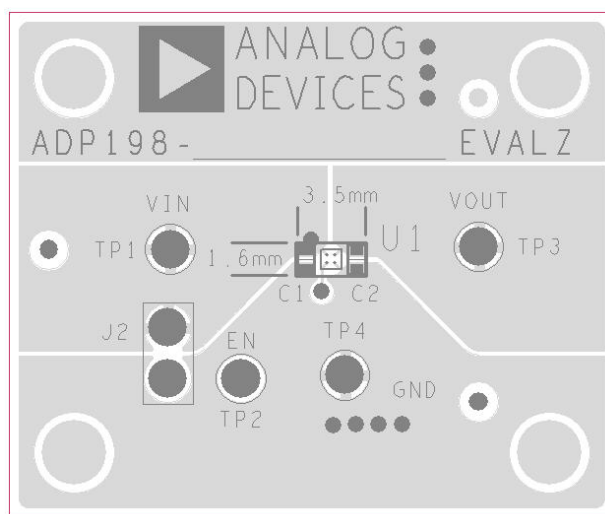
Figure 2. ADP198 WLCSP Evaluation Board
