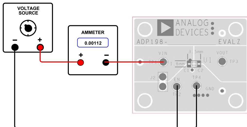
Figure 13. WLCSP Shutdown Current Measurement
