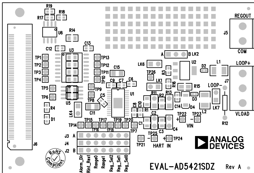
Figure 6. Component Placement Drawing
