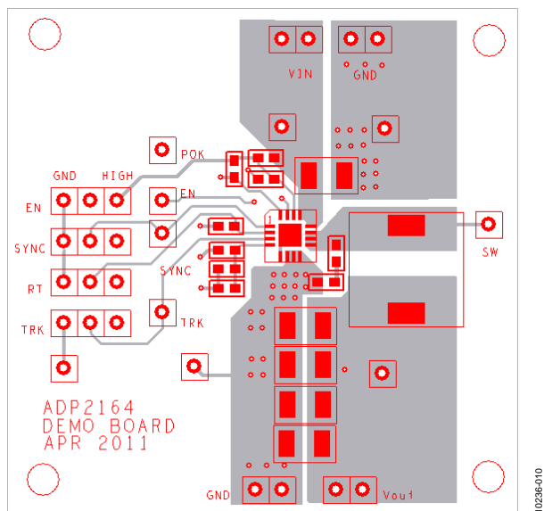
Figure 10. Top Layer
