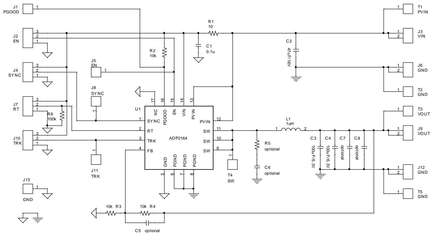
Figure 9. Schematic of the ADP2164 Evaluation Board
