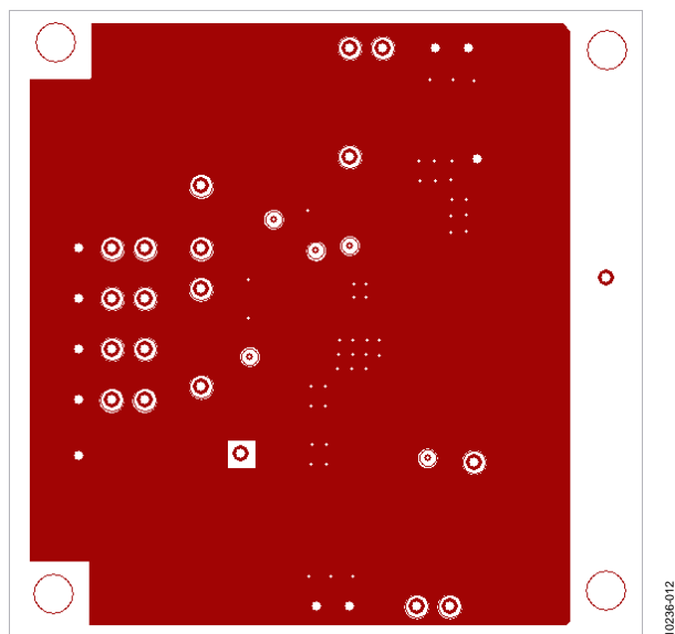
Figure 11. Third Layer
