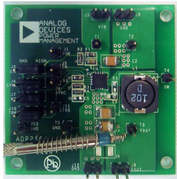
Figure 2. Output Ripple Measurement
