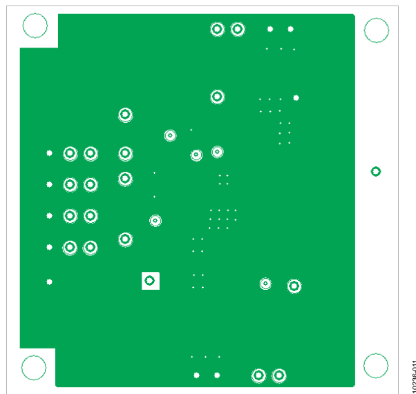
Figure 12. Second Layer
