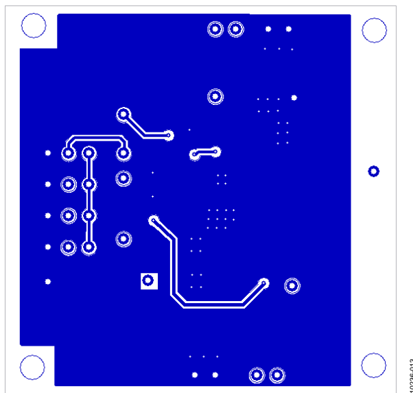
Figure 13. Bottom Layer
