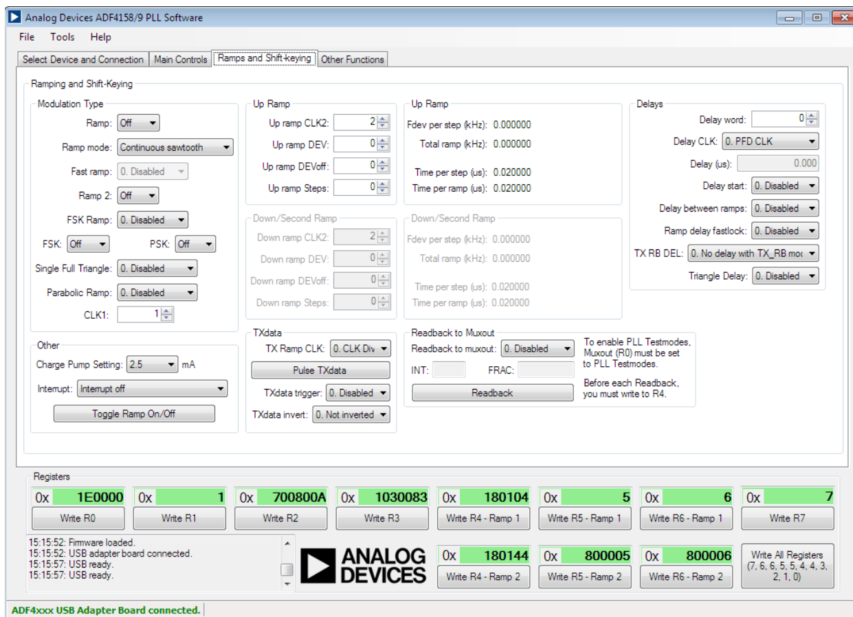
Figure 9. Software—Ramp Controls
