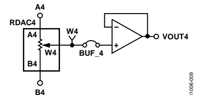
Figure 9. RDAC4
