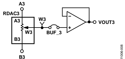
Figure 8. RDAC3
