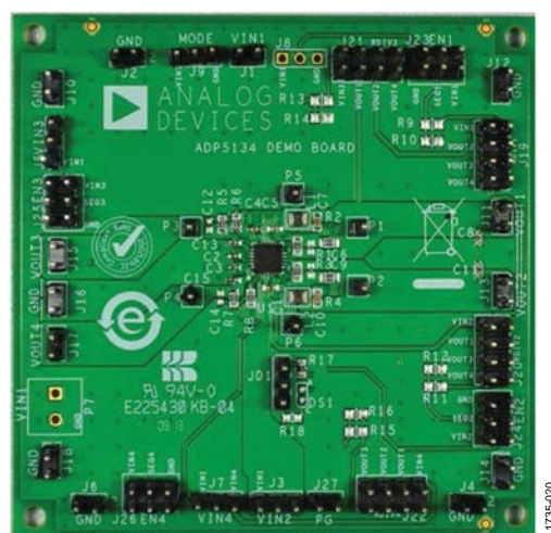
Figure 20. Evaluation Board for the ADP5134
