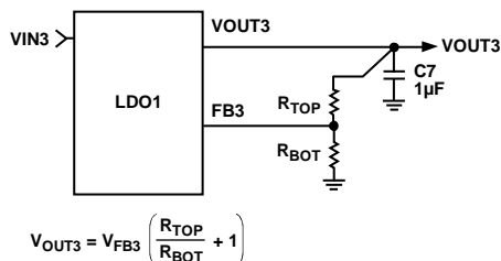
Figure 4. LDO1 External Output Voltage Setting
