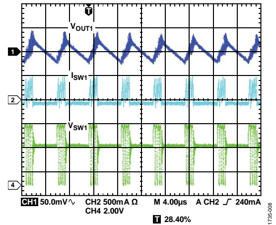
Figure 8. Typical Waveforms, V_{OUT1} = 3.3 V, I_{OUT1} = 30 mA, PSM Mode
