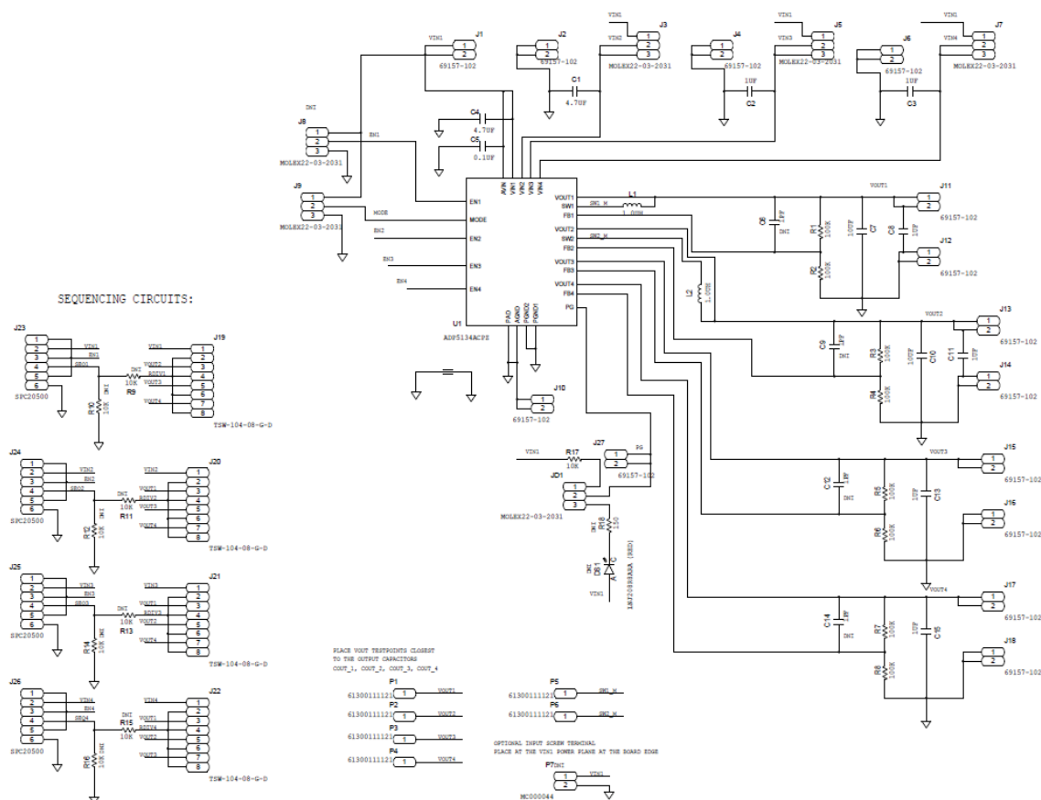
Figure 19. Evaluation Board Schematic of the ADP5134
