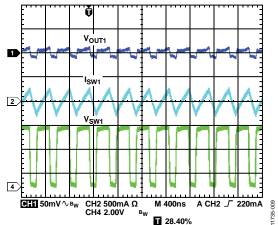
Figure 9. Typical Waveforms, V_{OUT1} = 3.3 V, I_{OUT1} = 30 mA, PWM Mode
