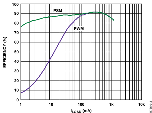
Figure 12. Buck Efficiency, V_{IN1} = 3.6V , V_{OUT1} = 1.8V
