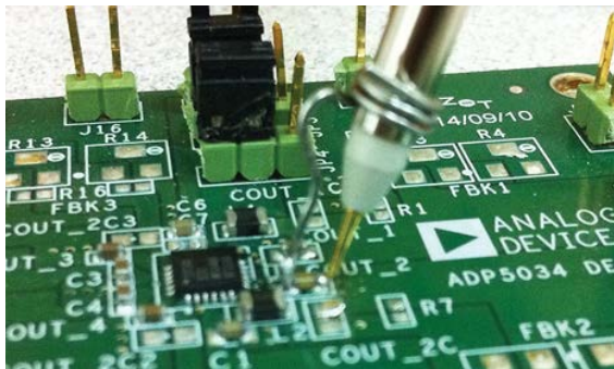
Figure 7. Measuring Output Voltage Ripple
