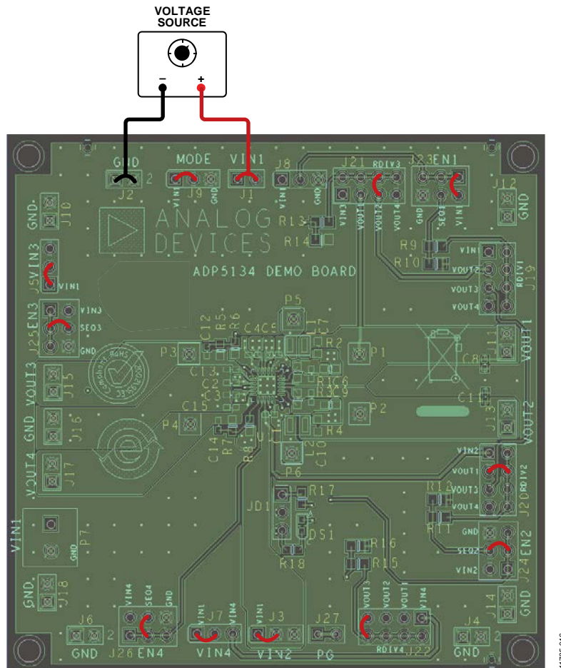
Figure 16. Regulators Connected in Sequence
