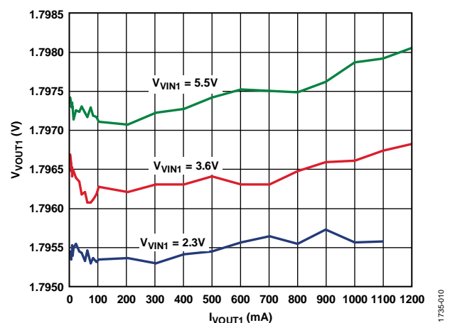
Figure 10. Buck Load Regulation
