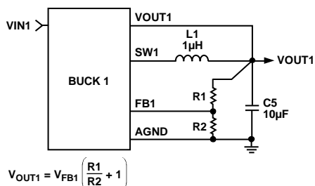
Figure 3. BUCK1 External Output Voltage Setting
