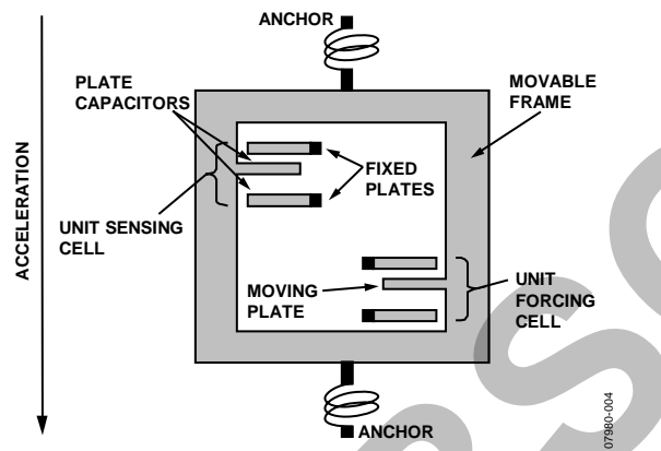
Figure 6. MEMS Sensor Diagram
