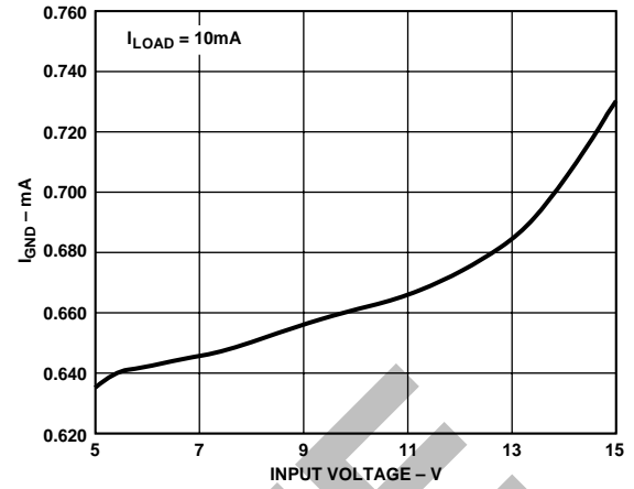
Figure 5. I_{GND} vs. V_{IN} ( I_{LOAD} = 10 mA )*
