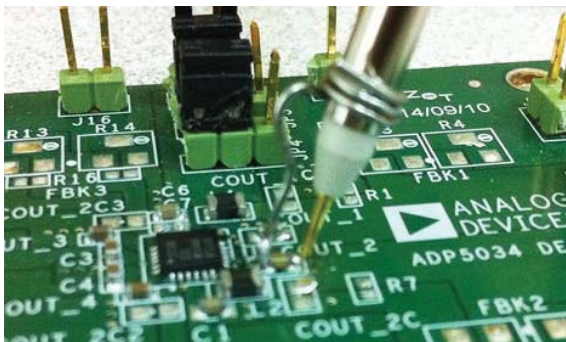
Figure 5. Measuring Output Voltage Ripple
