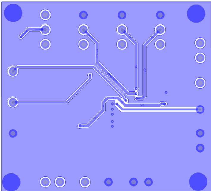
Figure 5. Second Layer
