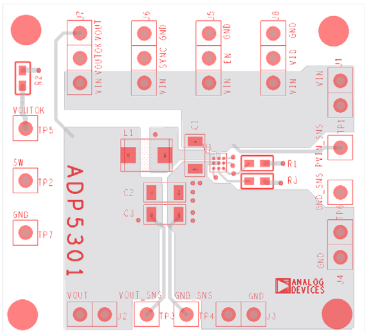
Figure 4. Top Layer
