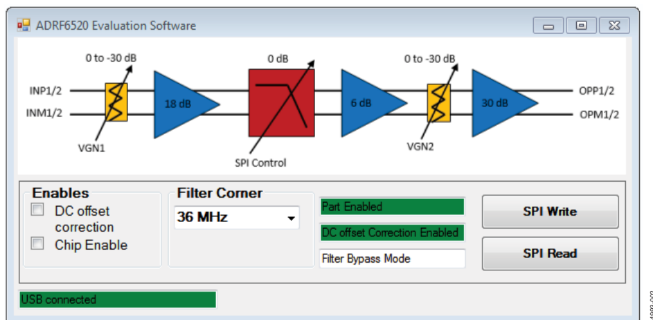
Figure 2. ADRF6520 Evaluation Software Graphical User Interface (GUI)
