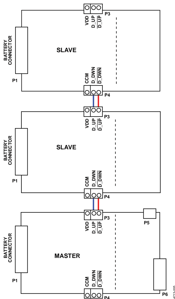
Figure 5. Configuration for Isolated Daisy Chain
