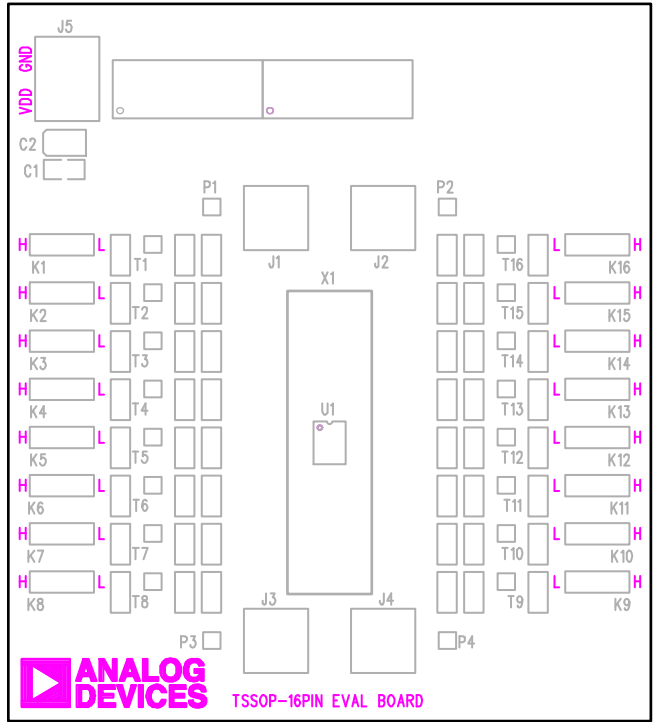
Figure 3. EVAL-16TSSOPEBZ Evaluation Board Silkscreen
