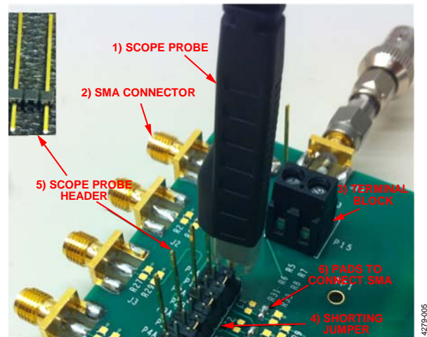
Figure 5. Optional Components
