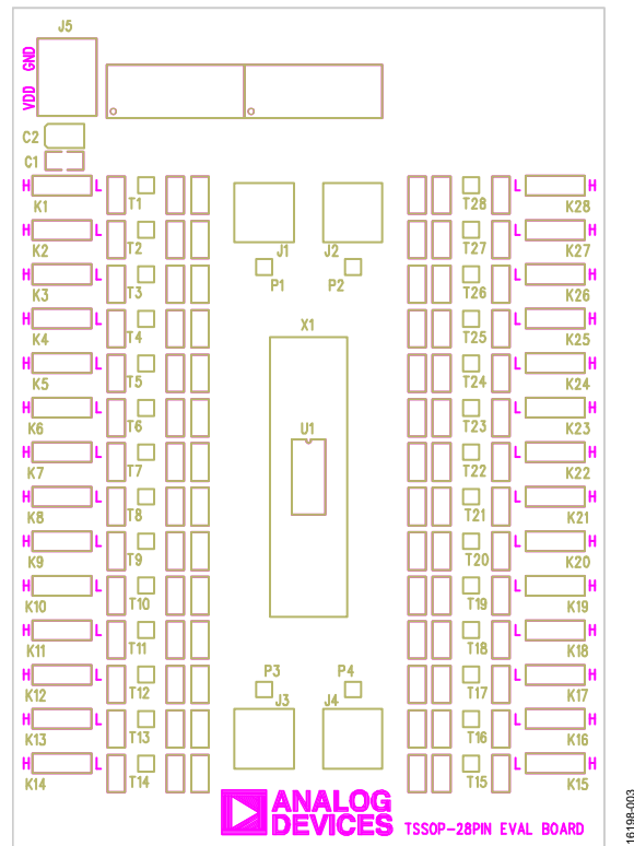
Figure 3. EVAL-28TSSOPEBZ Evaluation Board Silkscreen
