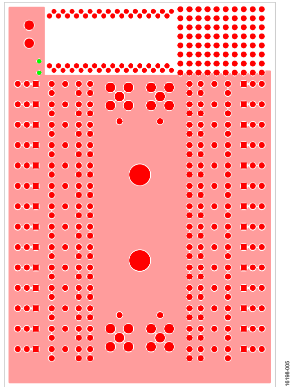
Figure 5. EVAL-28TSSOPEBZ Evaluation Board Bottom Layer
