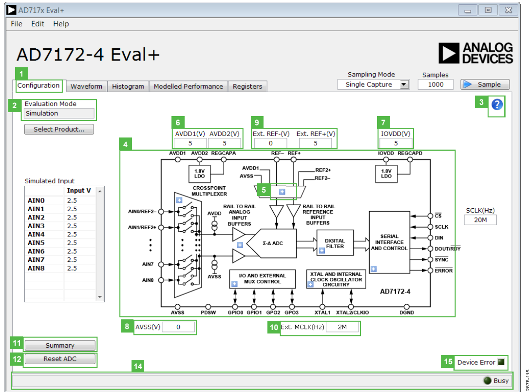
Figure 15. Configuration Tab of the AD7172x Eval+ Software in Hardware Mode
