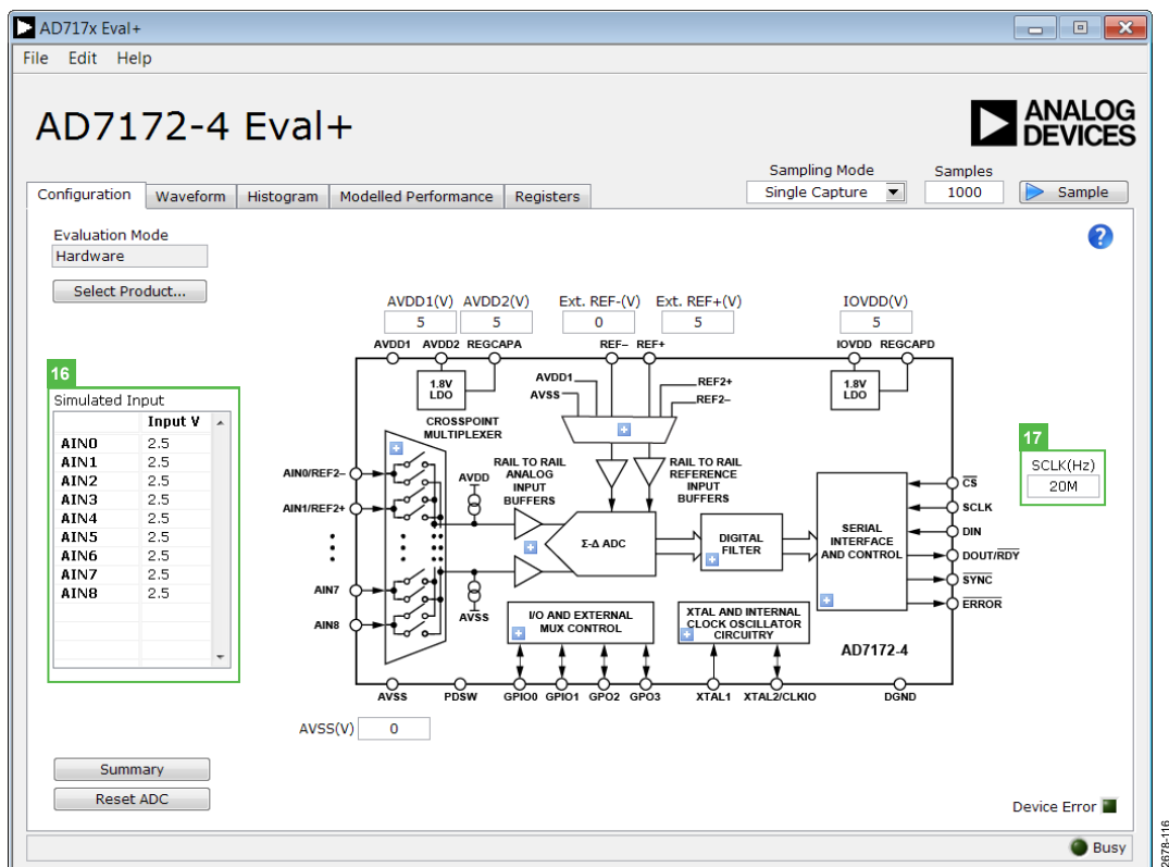
Figure 16. Configuration Tab of the AD7172-4 Evaluation Software in Simulation Mode
