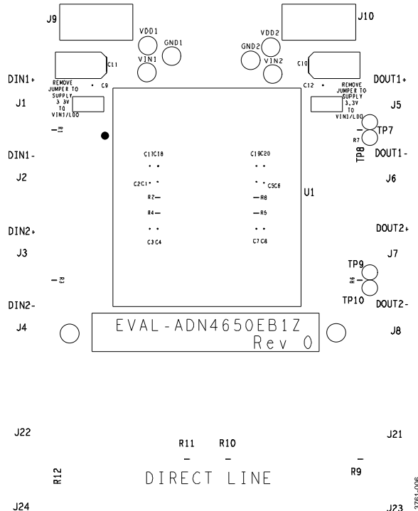
Figure 7. EVAL-ADN4650EB1Z Silkscreen
