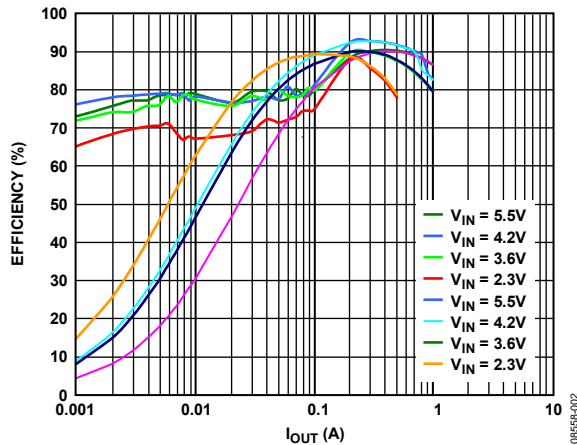
Figure 2. Efficiency vs. I_{OUT} , V_{OUT} = 3.3V , PWM and PSM
