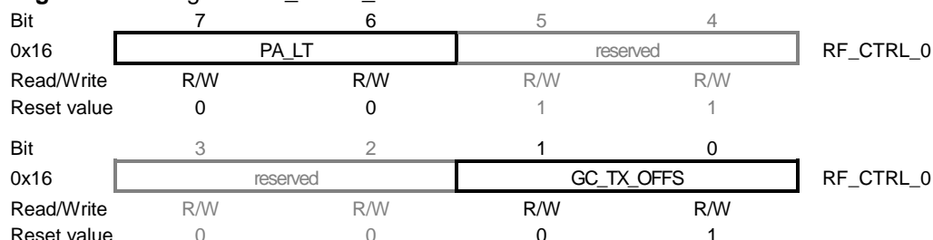
Figure 9-15. Register RF_CTRL_0.
