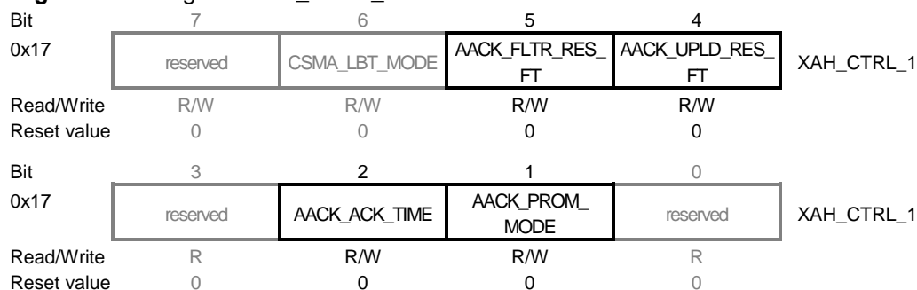
Figure 7-19. Register XAH_CTRL_1.
