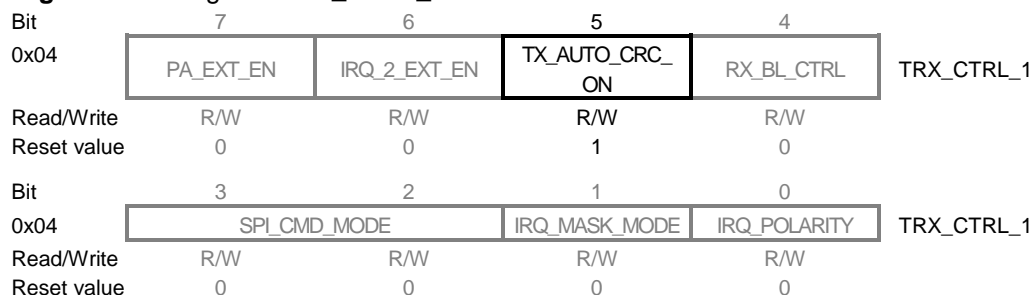
Figure 7-18. Register TRX_CTRL_1.
