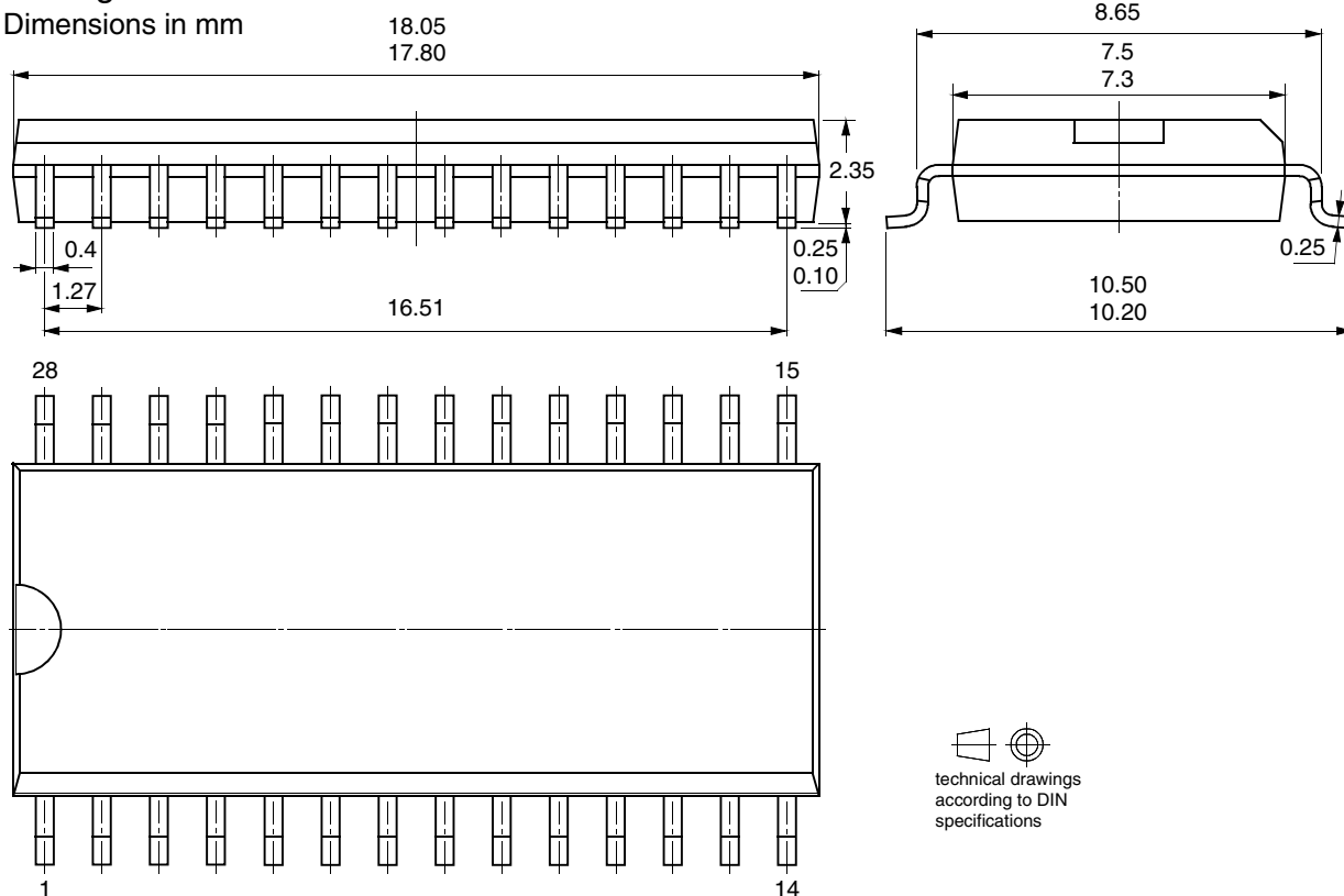
Figure 12-1. SO28
