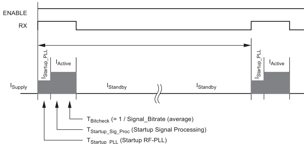
Figure 8-1. Polling Cycle
