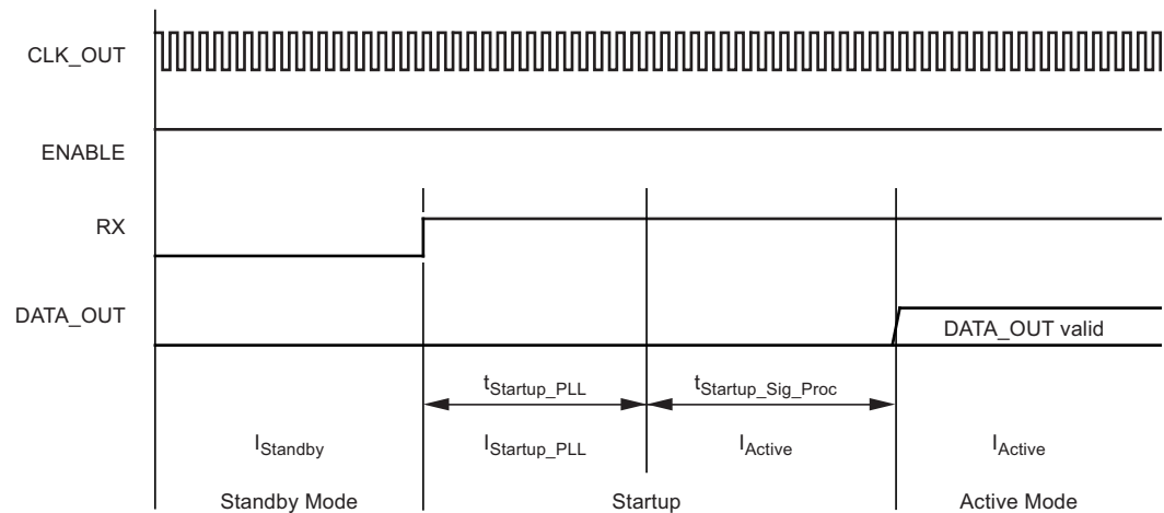
Figure 5-3. Active Mode
