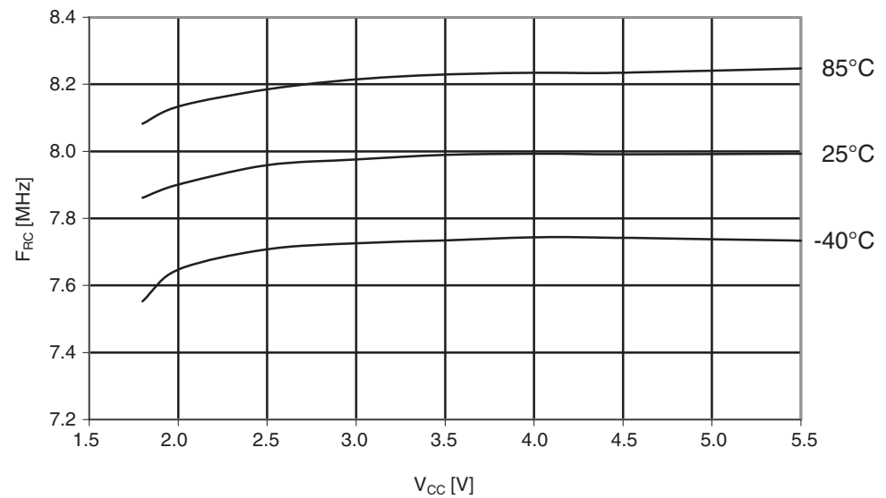
Figure 29-38. Atmel ATmega164A: Calibrated 8MHz RC oscillator vs. V_{CC} .
