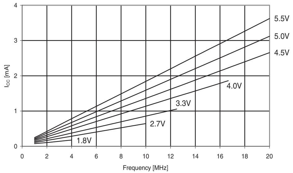
Figure 29-105. Atmel ATmega324A: Idle supply current vs. V_{CC} (1 - 20MHz).
