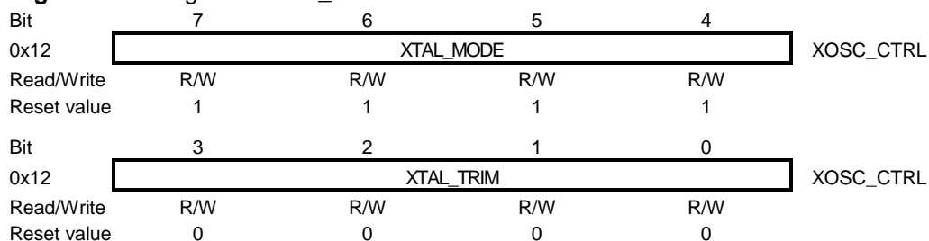
Figure 9-17. Register XOSC_CTRL.
