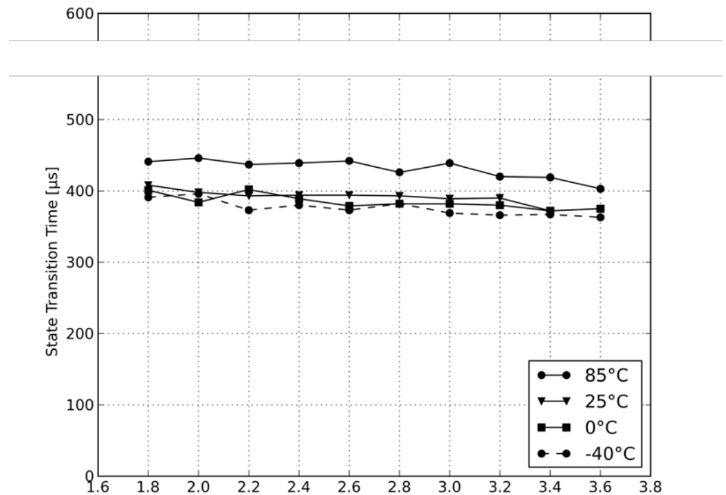
Figure 13-12. Transition Time from EVDD to P_ON (CLKM available).
