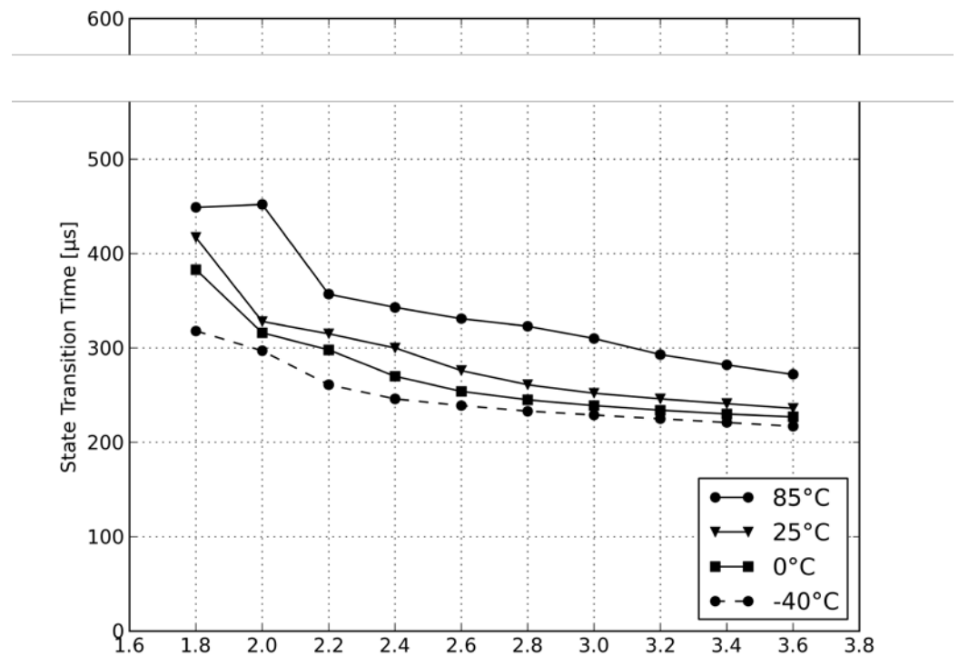
Figure 13-13. Transition Time from SLEEP to TRX_OFF (IRQ_4 (AWAKE_END)).
