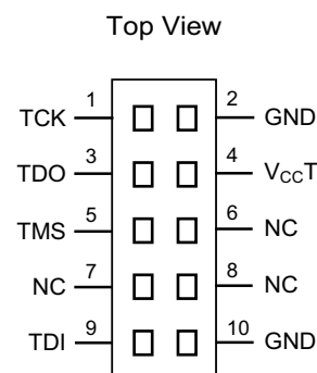
Figure 4. 10-pin Pinouts
