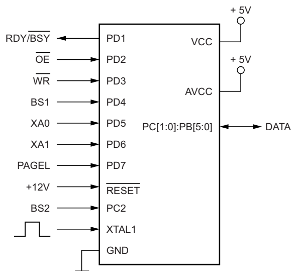
Figure 6-117. Parallel Programming
