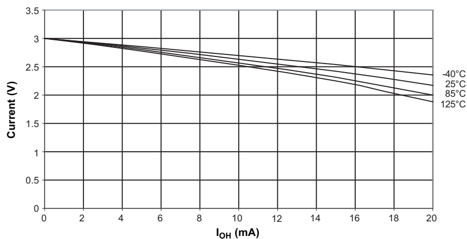
Figure 7-17. Output High Voltage versus Output High Current ( V_{CC} = 3V )
