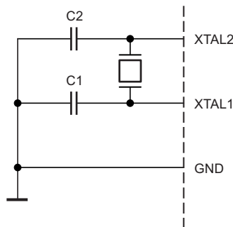
Figure 6-12. Crystal Oscillator Connections
