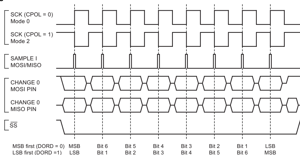
Figure 6-67. SPI Transfer Format with CPHA = 0
