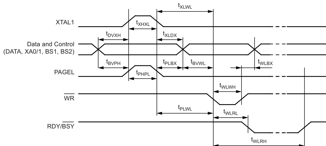
Figure 6-123. Parallel Programming Timing, Including some General Timing Requirements
