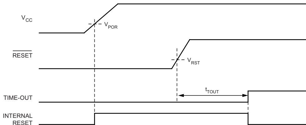
Figure 6-17. MCU Start-up, \overline{\text{RESET}} Extended Externally
