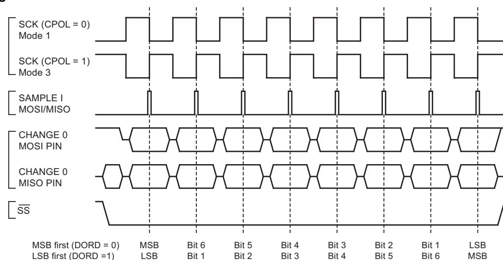
Figure 6-68. SPI Transfer Format with CPHA = 1
