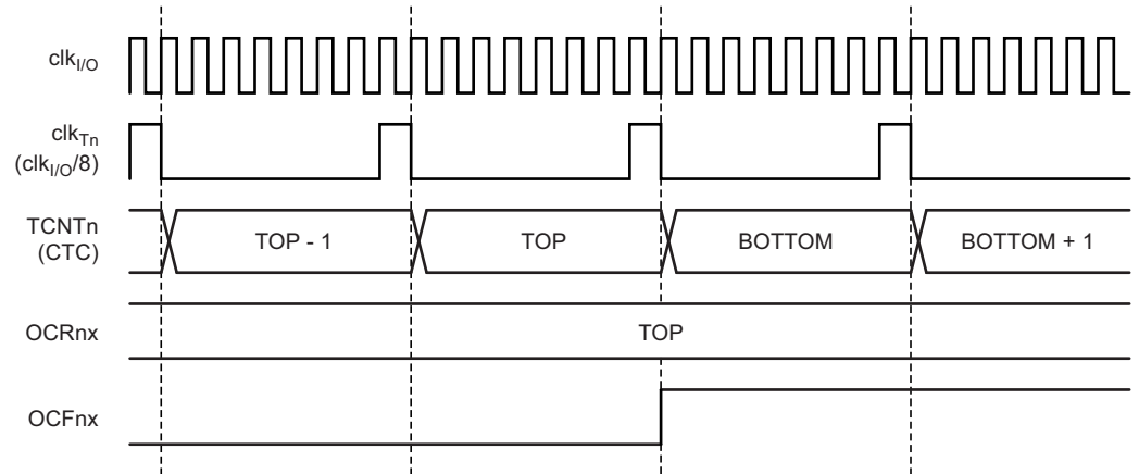
Figure 6-37. Timer/Counter Timing Diagram, Clear Timer on Compare Match Mode, with Prescaler ( f_{clk\_I/O}/8 )
