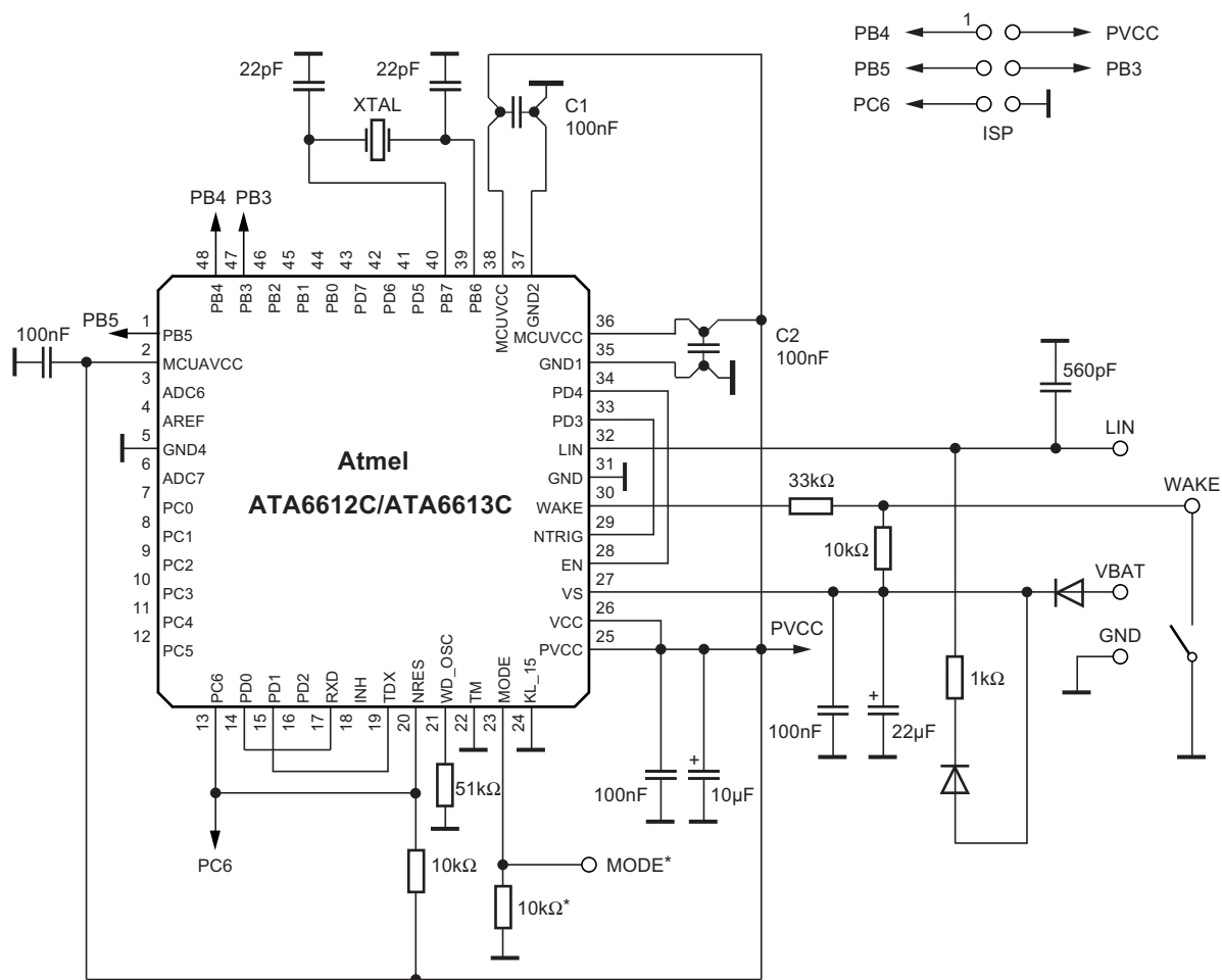
Figure 8-2. Typical LIN Master Application
