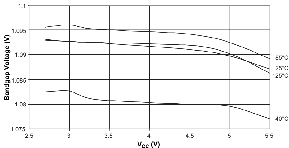
Figure 7-29. Bandgap Voltage versus V_{CC}
