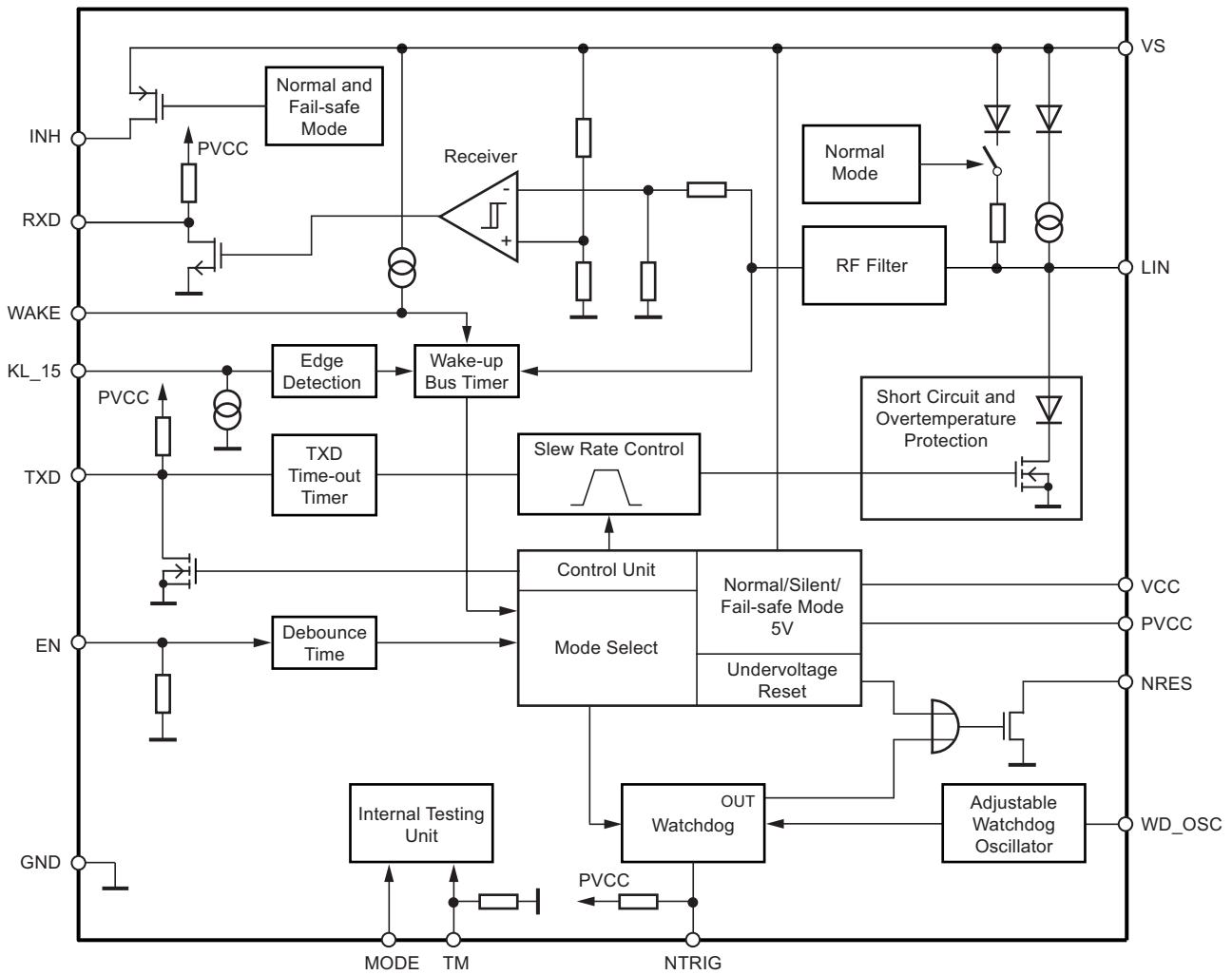
Figure 4-1. Block Diagram
