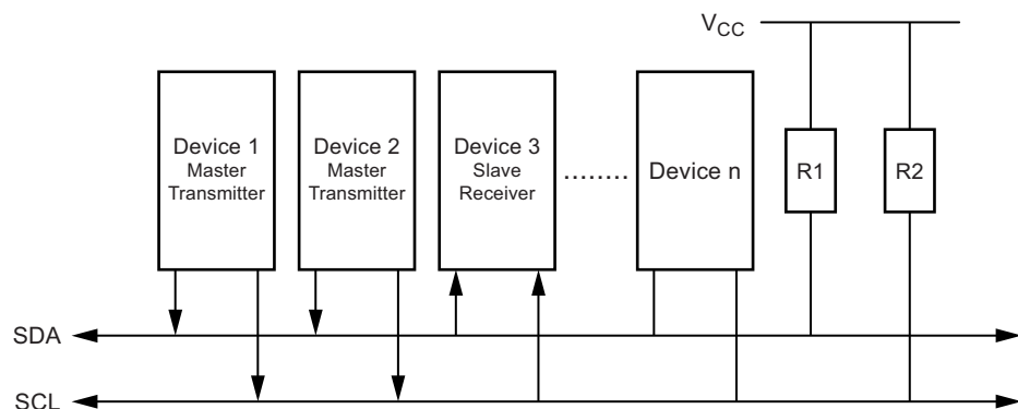
Figure 6-97. An Arbitration Example
