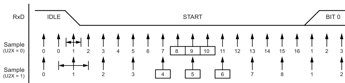
Figure 6-73. Start Bit Sampling
