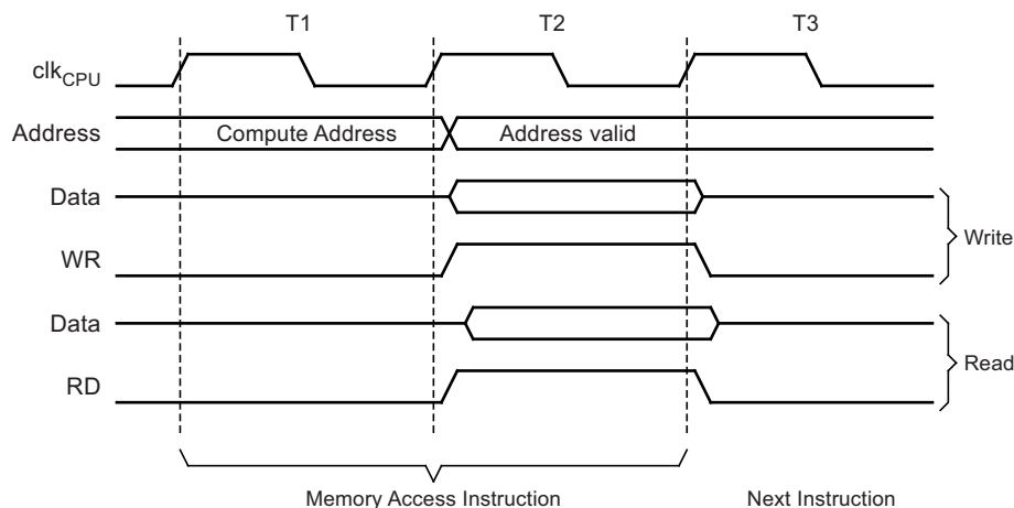
Figure 6-10. On-chip Data SRAM Access Cycles
