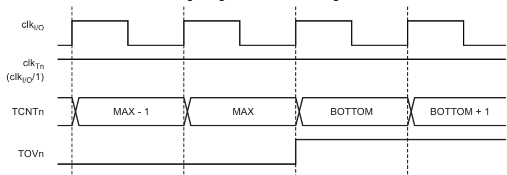
Figure 6-60. Timer/Counter Timing Diagram, no Prescaling
