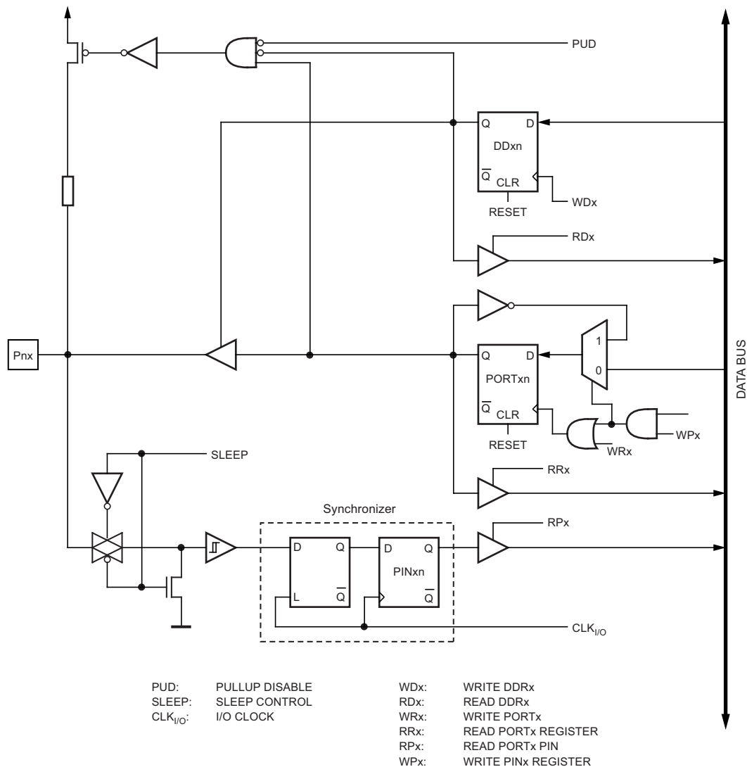
Figure 6-23. General Digital I/O (1)
