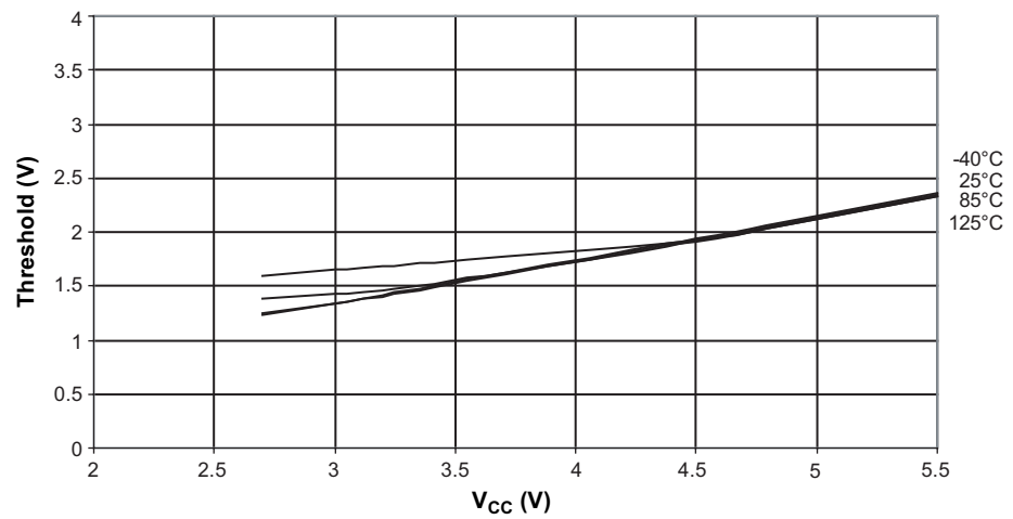
Figure 7-20. Reset Input Threshold Voltage versus V_{CC} (VIH, Reset Pin Read as 1)
