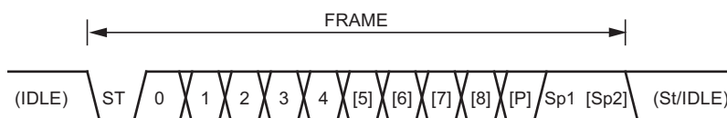
Figure 6-72. Frame Formats
