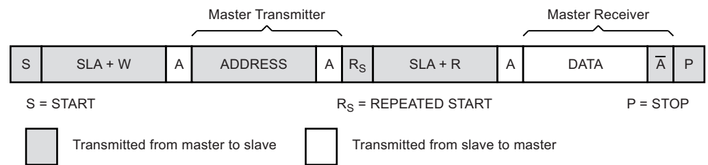
Figure 6-96. Combining Several TWI Modes to Access a Serial EEPROM
