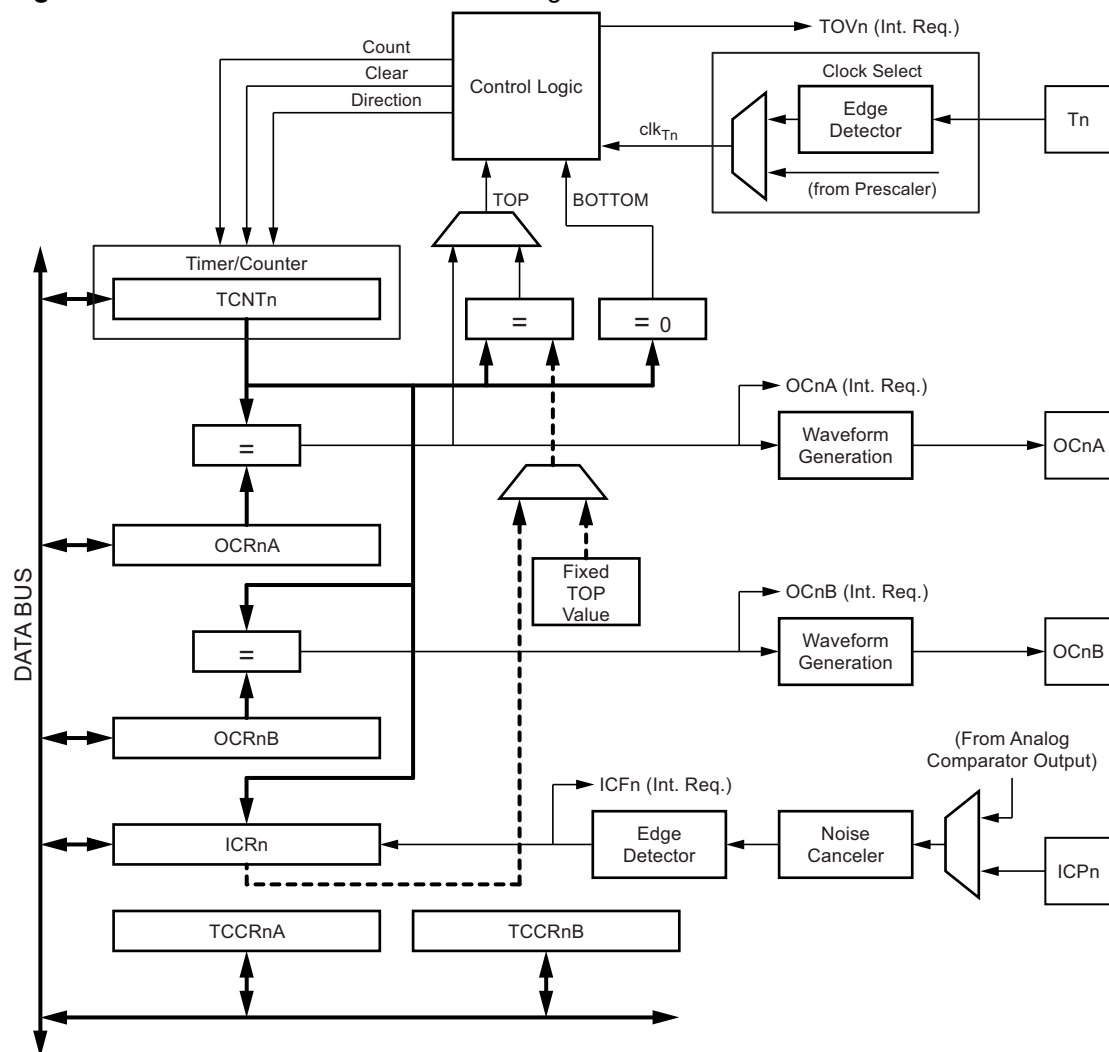
Figure 6-40. 16-bit Timer/Counter Block Diagram (1)
