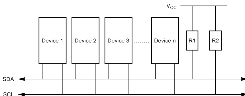
Figure 6-77. TWI Bus Interconnection
