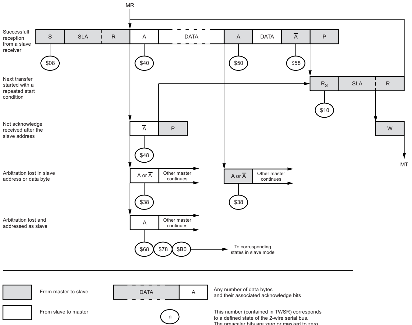
Figure 6-91. Formats and States in the Master Receiver Mode
