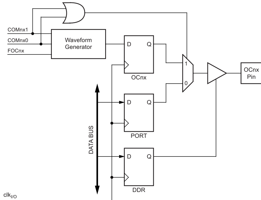
Figure 6-56. Compare Match Output Unit, Schematic
