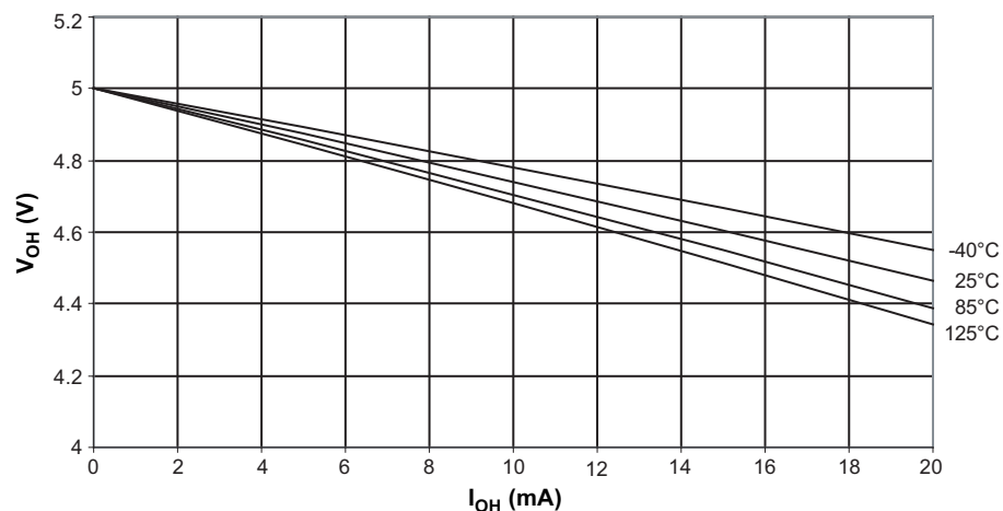
Figure 7-11. Output High Voltage vs. Output High Current ( V_{CC} = 5V )
