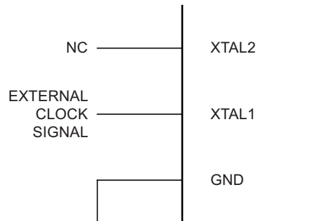
Figure 6-14. External Clock Drive Configuration
