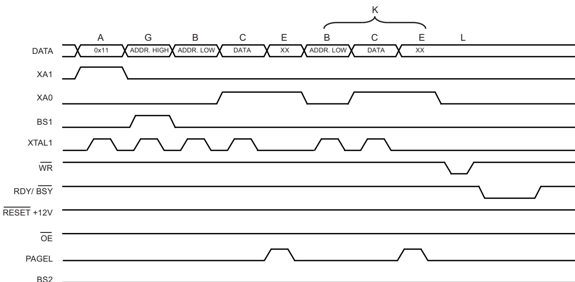
Figure 6-120. Programming the EEPROM Waveforms
