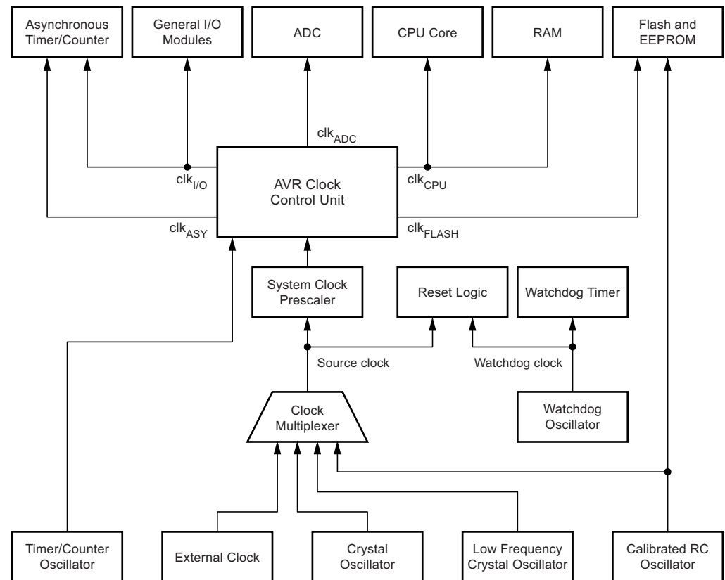
Figure 6-11. Clock Distribution
