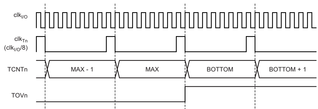
Figure 6-35. Timer/Counter Timing Diagram, with Prescaler ( f_{\text{clk\_I/O}}/8 )
