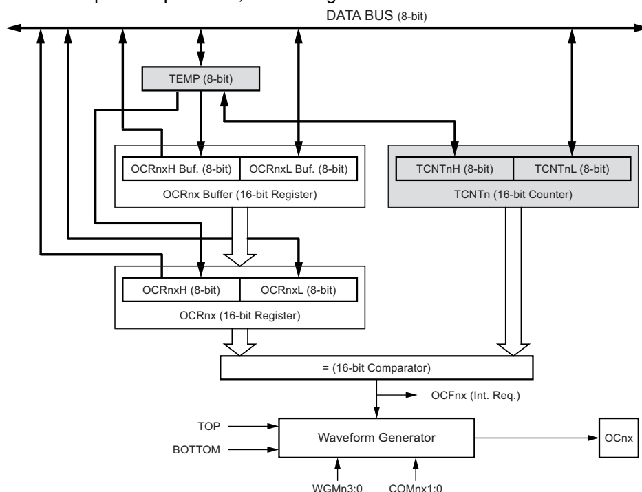
Figure 6-43. Output Compare Unit, Block Diagram
