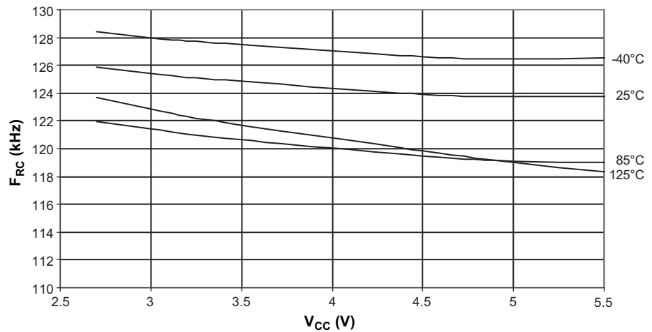
Figure 7-22. Watchdog Oscillator Frequency vs. V_{CC}
