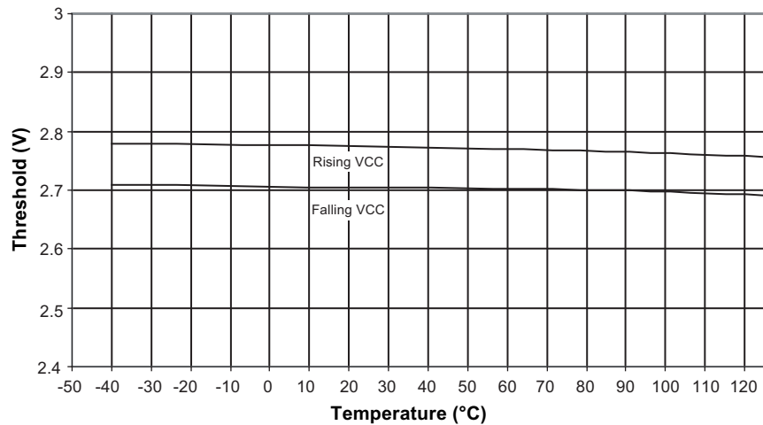
Figure 7-28. BOD Threshold versus Temperature (BODLEVEL is 2.7V)
