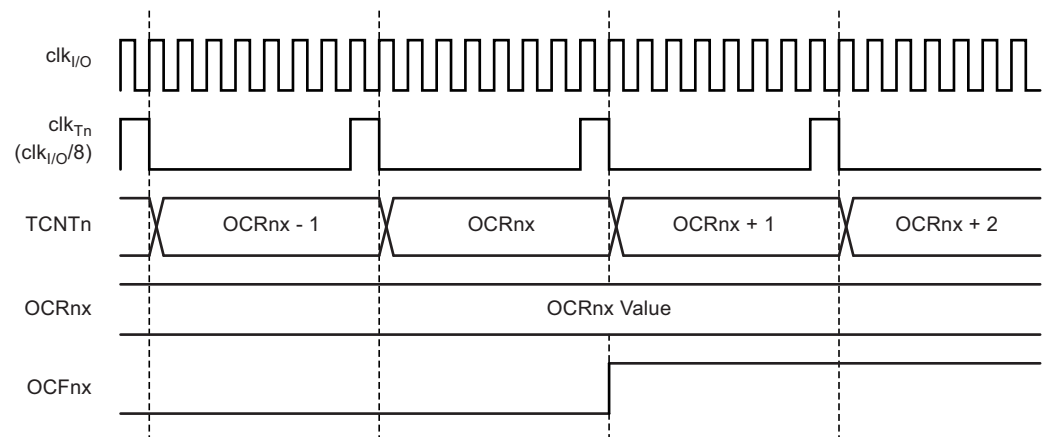
Figure 6-50. Timer/Counter Timing Diagram, Setting of OCF1x, with Prescaler ( f_{clk\_I/O}/8 )
