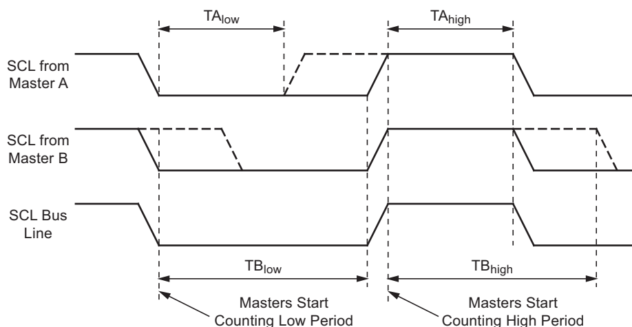
Figure 6-83. SCL Synchronization Between Multiple Masters
