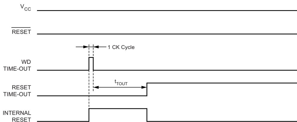
Figure 6-20. Watchdog System Reset During Operation
