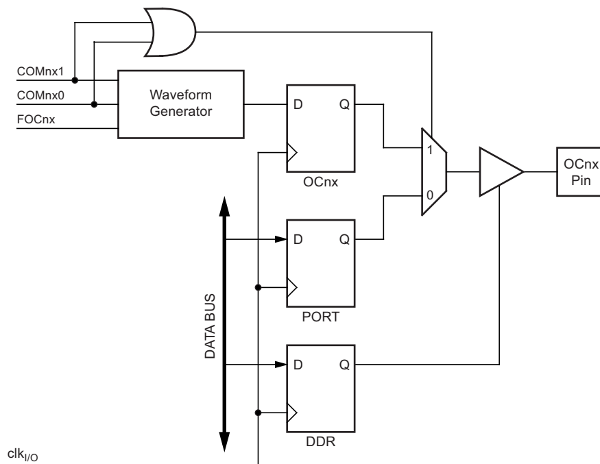
Figure 6-44. Compare Match Output Unit, Schematic
