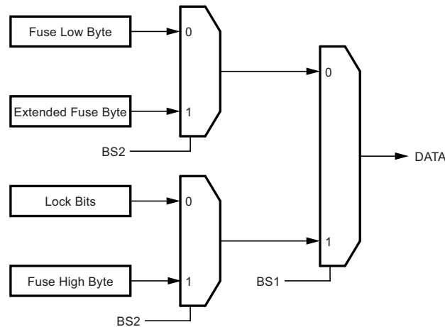
Figure 6-122. Mapping Between BS1, BS2 and the Fuse and Lock Bits During Read
