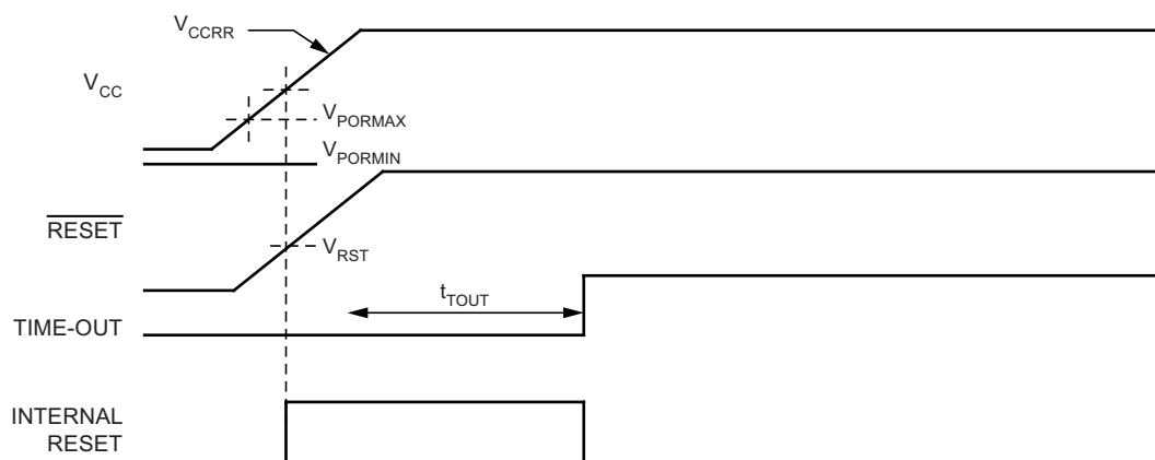
Figure 6-16. MCU Start-up, \overline{\text{RESET}} Tied to V_{CC}
