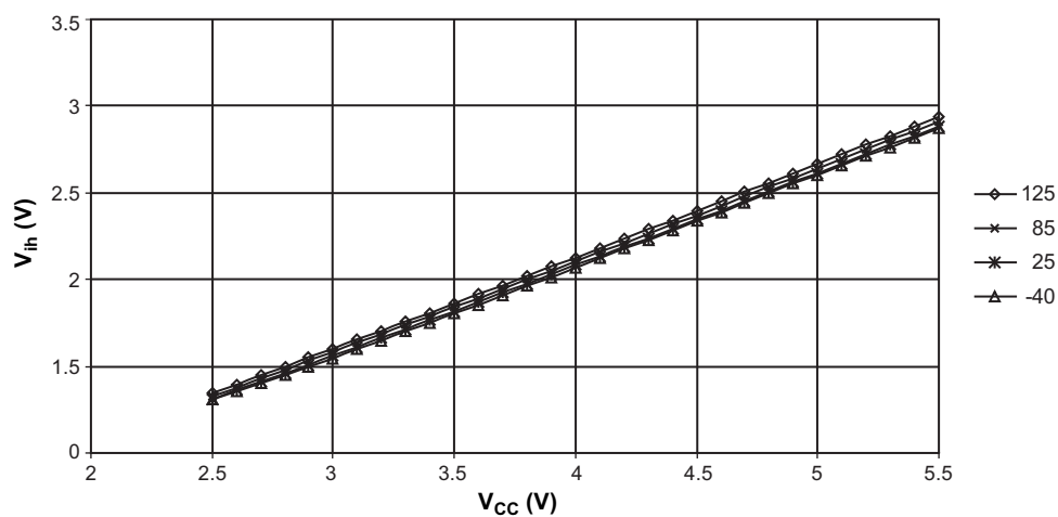
Figure 7-18. I/O Pin Input Threshold versus V_{CC} ( V_{IH} , I/O Pin Read as 1)
