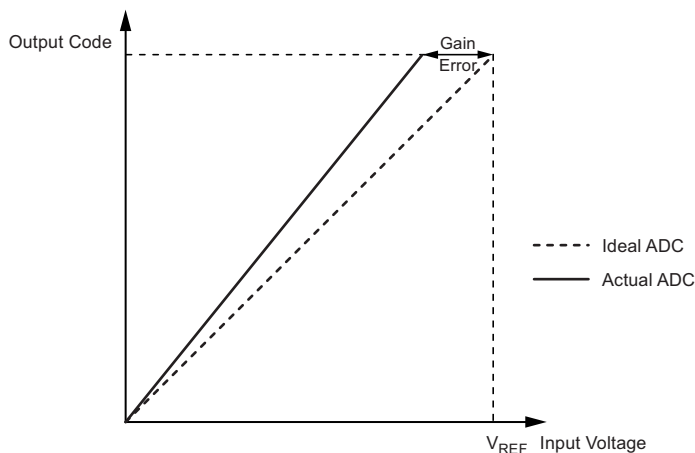
Figure 6-110. Gain Error
