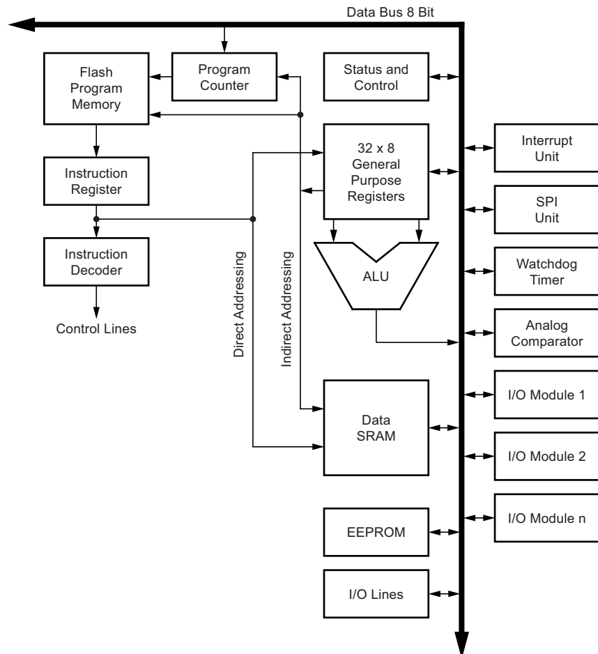
Figure 6-2. Block Diagram of the Atmel AVR Architecture
