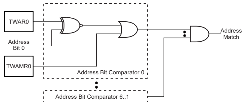
Figure 6-86. TWI Address Match Logic, Block Diagram
