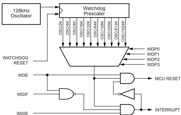
Figure 6-21. Watchdog Timer
