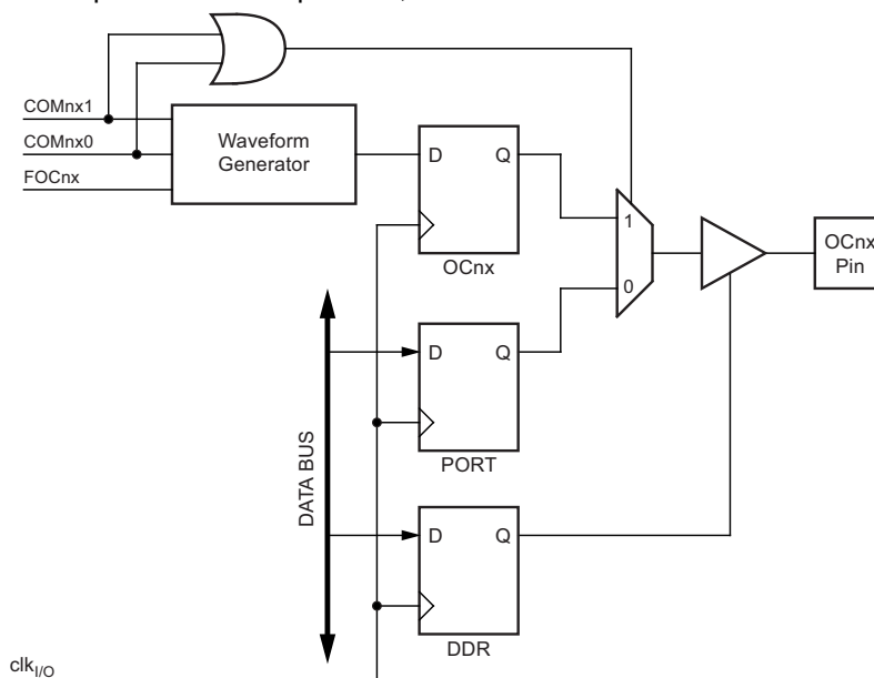
Figure 6-30. Compare Match Output Unit, Schematic
