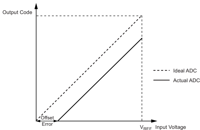
Figure 6-109. Offset Error
