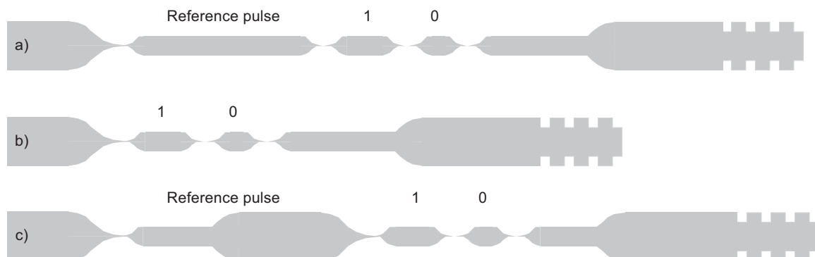
Figure 5-13. Long-leading-reference Protocol
