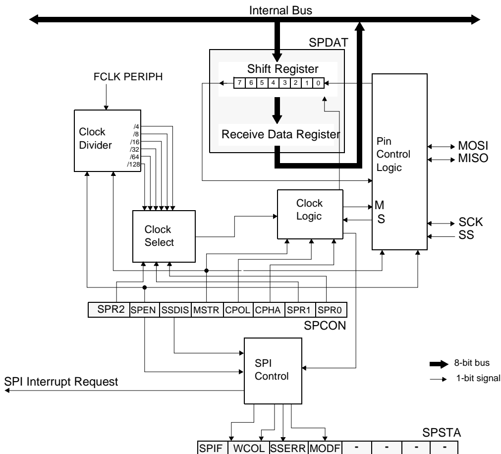
Figure 40. SPI Module Block Diagram
